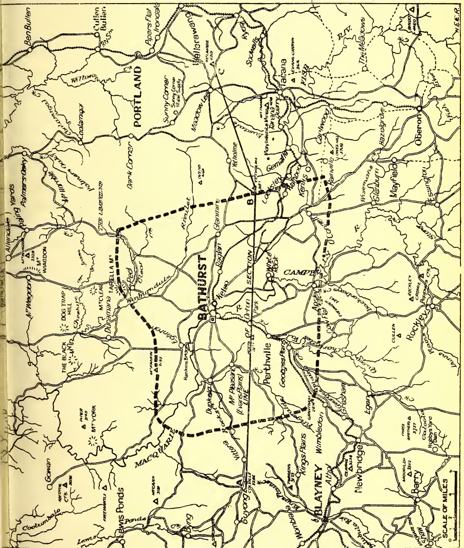
Area of the Bathurst Senkungsfeld shown by broken line
