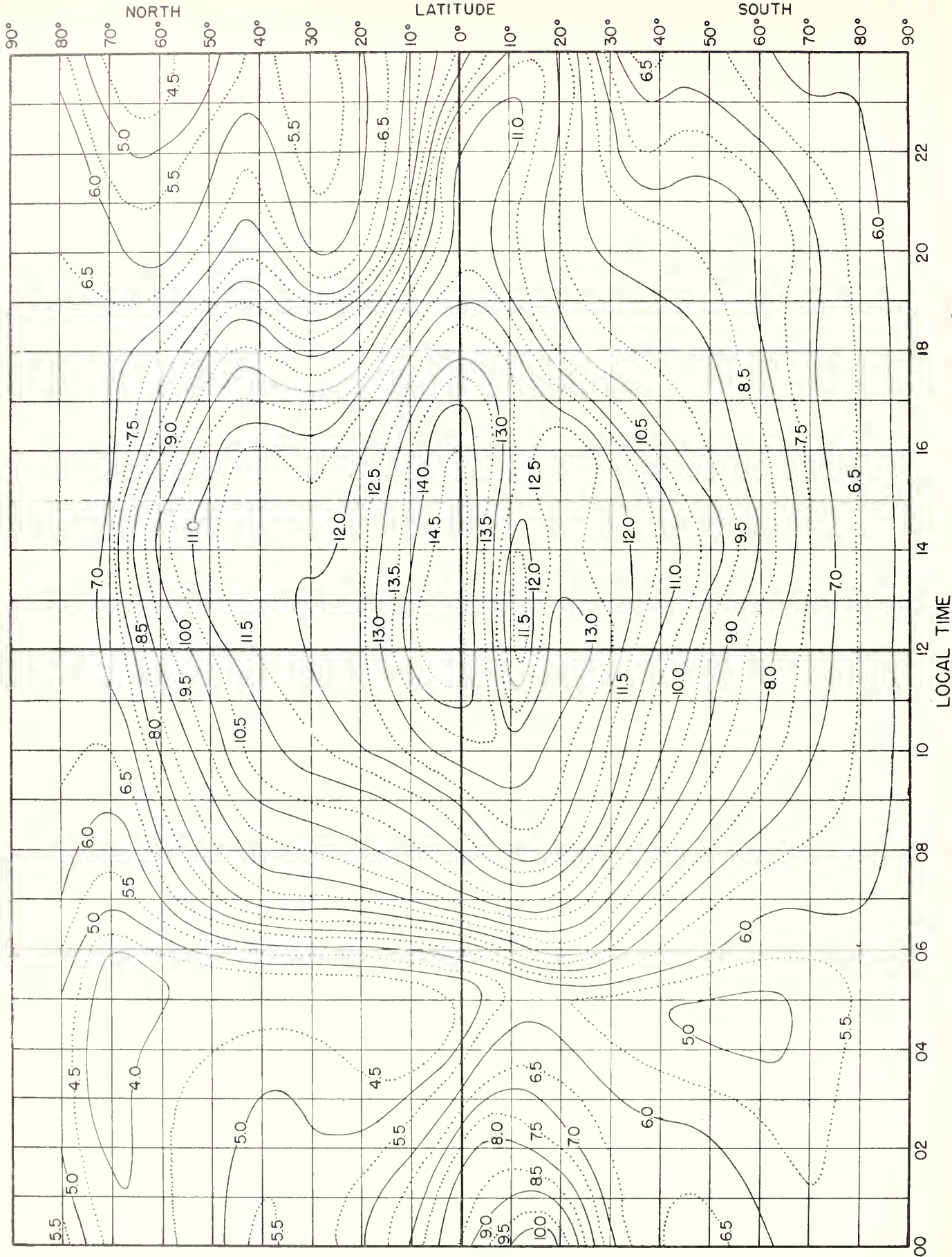
Fig. 5. F_2 ZERO - MUF, IN Mc, W ZONE, PREDICTED FOR OCTOBER, 1946.
