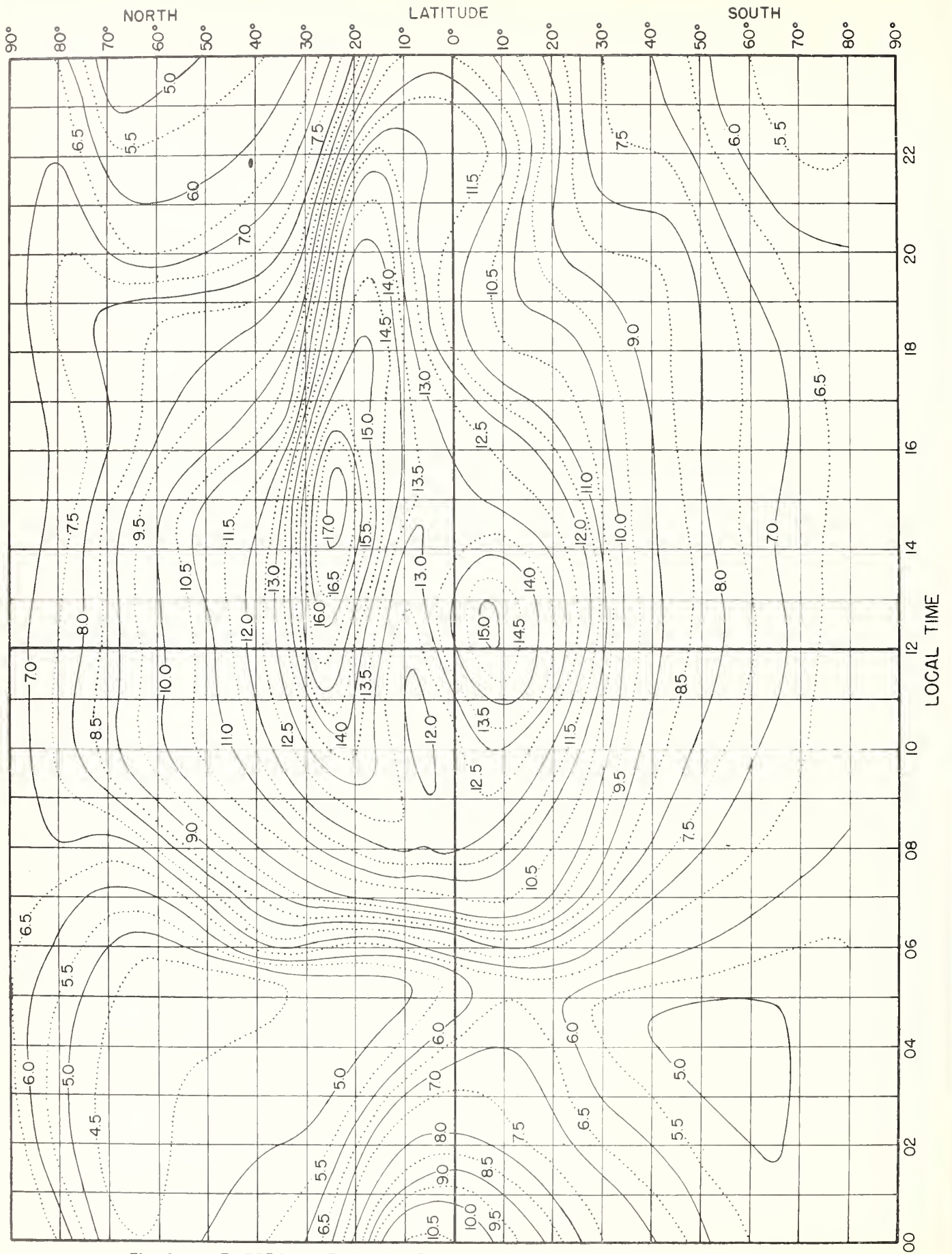
Fig. 9. F_2 ZERO-MUF, IN Mc, E ZONE, PREDICTED FOR OCTOBER, 1946.
