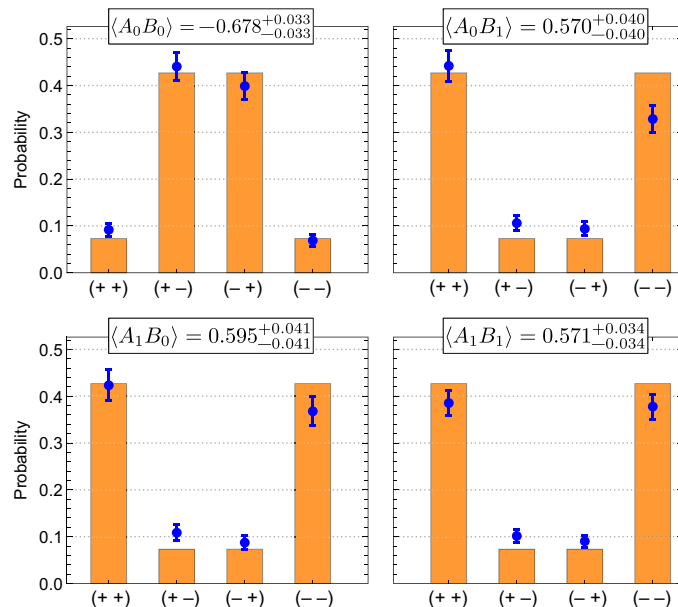
Fig. 3. Experimental data. The outcome probabilities comprising each of the four expectation values \langle A_0 B_0 \rangle, \langle A_0 B_1 \rangle, \langle A_1 B_0 \rangle , and \langle A_1 B_1 \rangle are obtained from the measured sixfold coincidence events for each set of 4 \times 4 eigenvectors during a fixed time window. Shown here are only the data corresponding to nonzero eigenvalues labeled on the horizontal axes + and - for +1 and -1, respectively, with the full data shown in the Supplementary Materials. The theoretical predictions are shown as orange bars, and each measured expectation value is given above the corresponding subfigure. Uncertainties on the latter and error bars on the data represent 1\sigma statistical confidence intervals assuming Poissonian counting statistics (see the Supplementary Materials).
