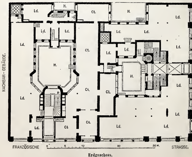
Erdgeschoss.
