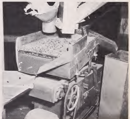
FIGURE 12.— A shaker machine used to separate stones from farmers' stock peanuts. The stones are discharged into the containers at the right and the peanuts come off the chute at the left.
