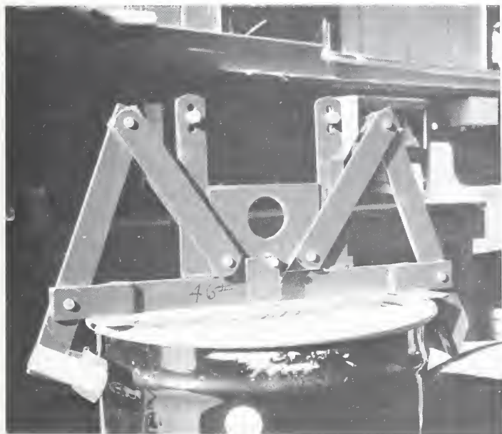
Figure 28. Barrel-lifting device.
