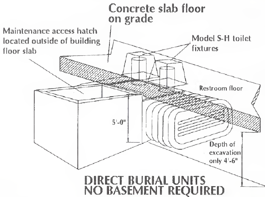
Figure 21. Bio-Sun dehydrating/composting tank schematic.
