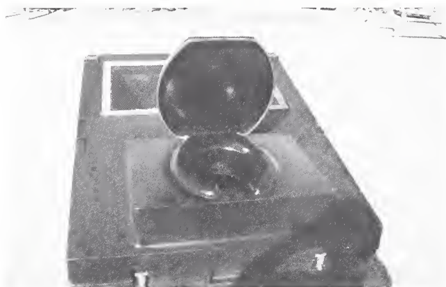
Figure 19 "Trail Site" composter by Romtec. The seat is an integral part of the unit. This unit is designed for just a privacy screen.
