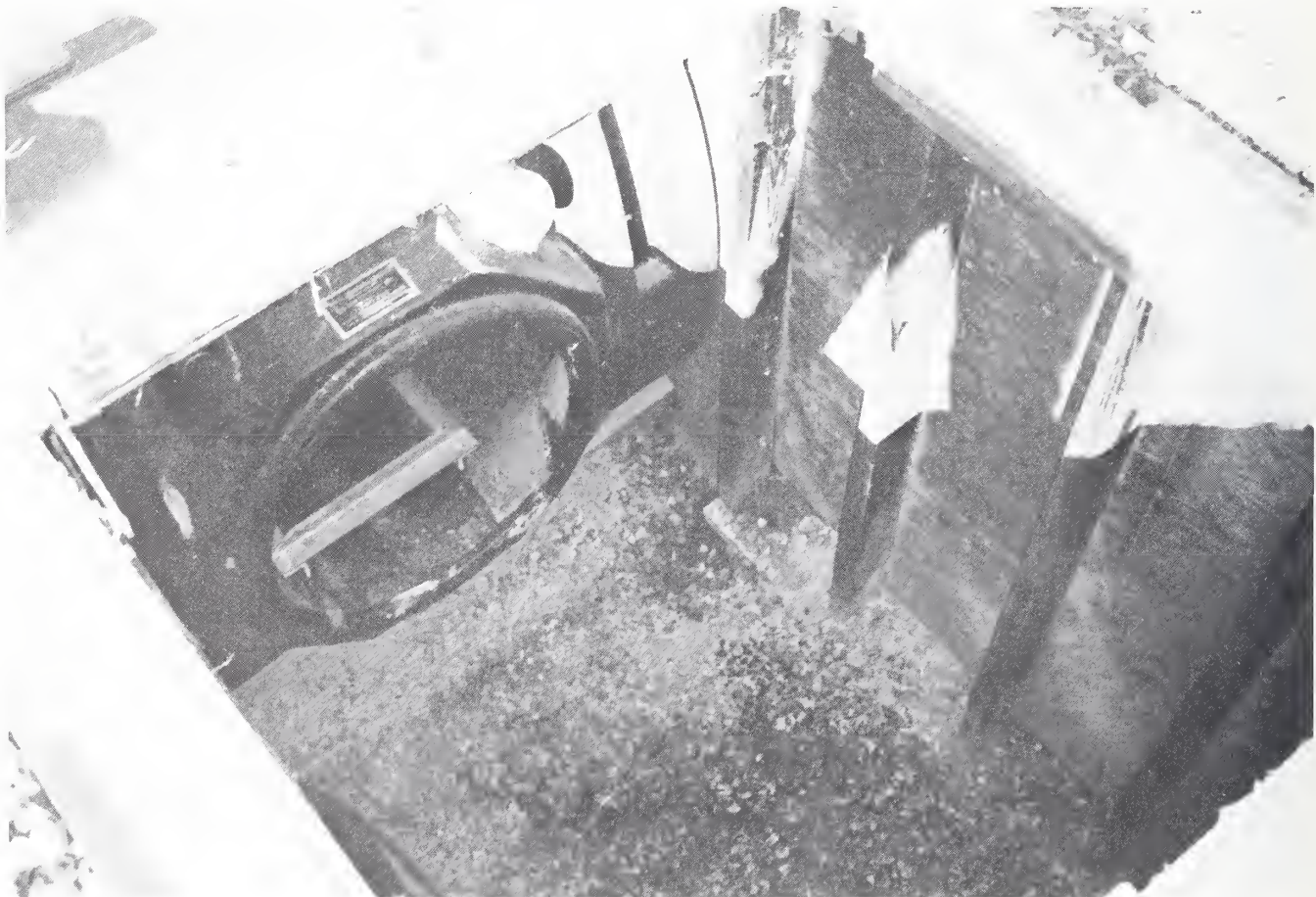
Figure 22. Bio-Sun dehydrating/composting tank viewed through open access hatch.
