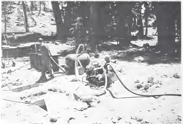
Figure 26. Pumping a septic tank. The sludge is pumped with the aid of a vacuum tank.
