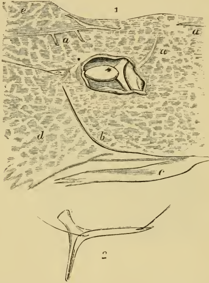
FIG. 7. — Poison Organ of Thalassophryne reticulata (after Günther). 1, Hinder half of the head with the venom-sac of the opercular apparatus in situ . * Place where the small opening in the sac has been observed. a , Lateral line and its branches; b , gill-opening; c , central fin; d , base of pectoral fin; e , base of dorsal fin 2, Operculum, with the perforated spine.
