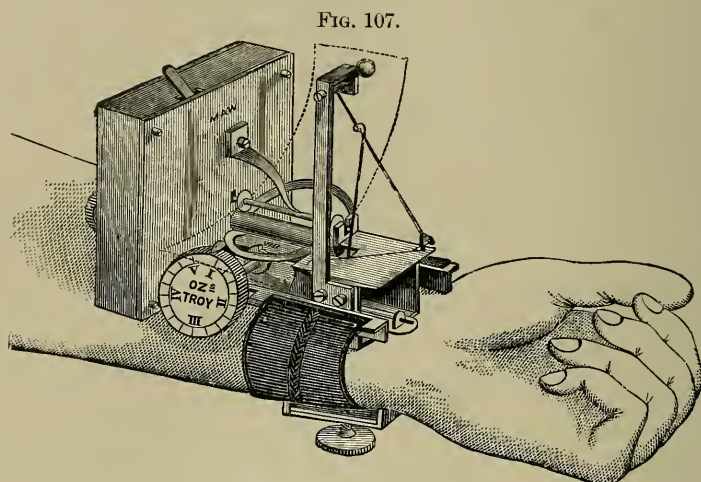
Dudgeon's sphygmograph.
