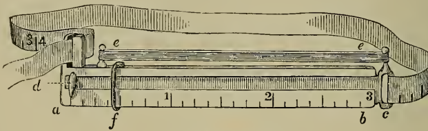
Carroll's stethometer.
