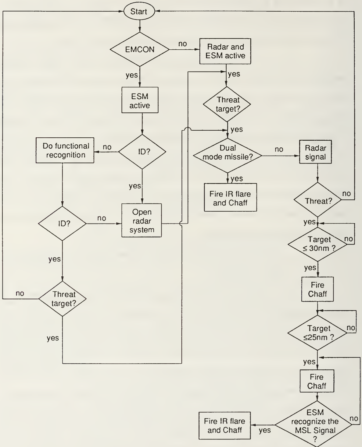
Figure 2.7: A Basic Procedure for Firing a Chaff and IR Flare
