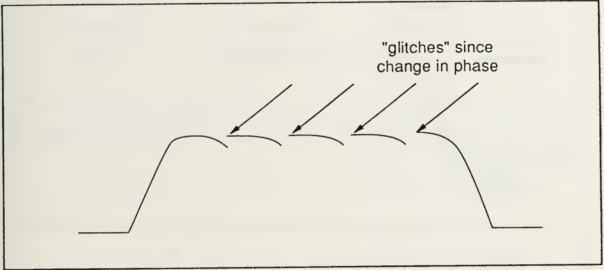
Figure 2.9: Phase Modulation Radar Pulse on an Oscilloscope
