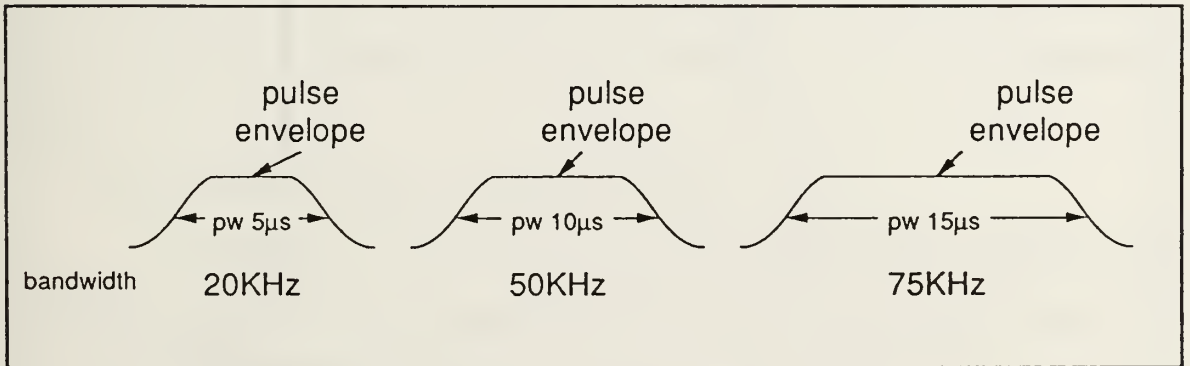
Figure 2.10: Select Different Bandwidths on an ESM Receiver to Identify Frequency Modulation Radar; PW varies with Different Bandwidth selected
