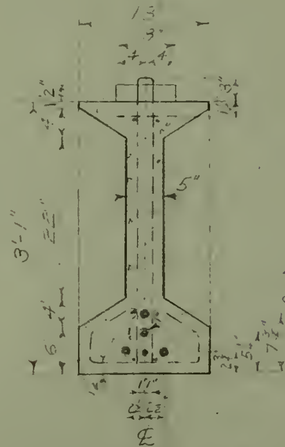
SECTION AT E SCALE \frac{3}{4} " = 1'-0"
