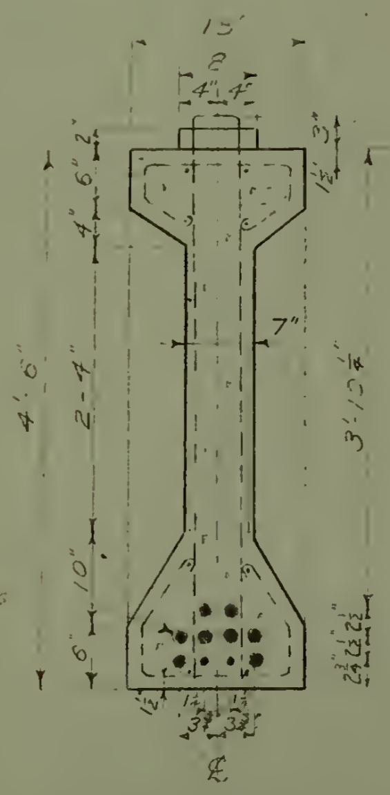
SECTION AT C SCALE \sim \frac{3}{4}'' 1'-0''
