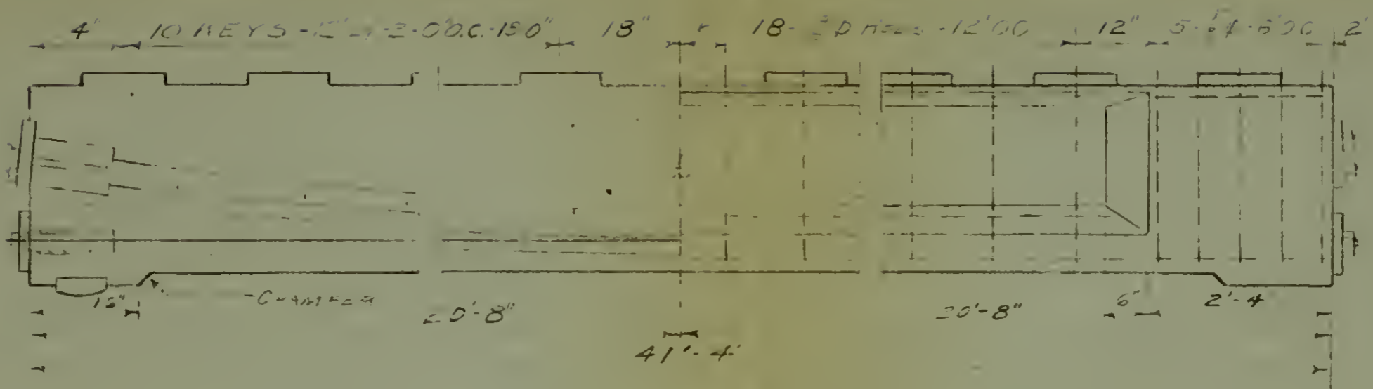
ELEVATION SCALE 1/4" = 1'-0"
