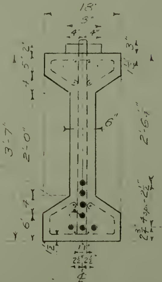
SECTION AT \phi SCALE \frac{1}{4} " = 1'-0"
