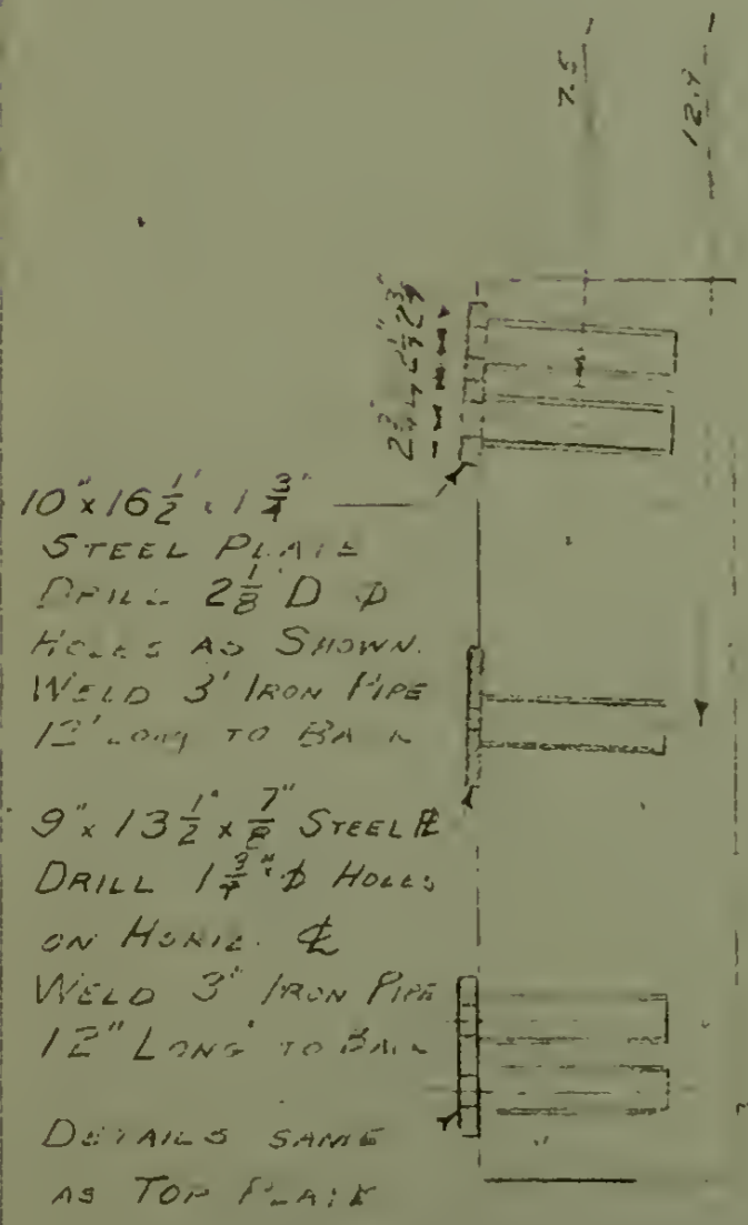
BEARING & DETAILS SCALE \sim \frac{3}{4}'' 1'-0''
