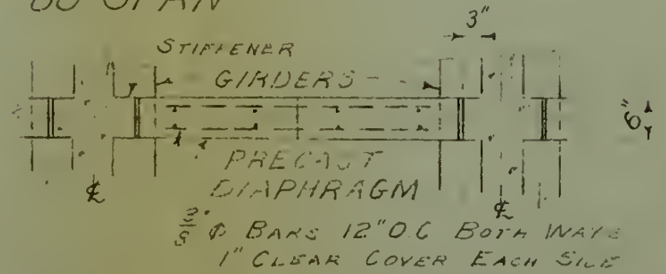
FIGURE No. 4 STANDARD DECK AND DIAPHRAGM DETAILS
