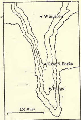
FIG. 210.—Some of the shore lines of Lake Agassiz. (After Upham, U. S. Geological Survey.)
