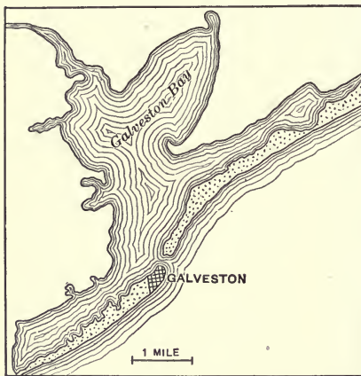
FIG. 245.—Barrier beaches on the Texas coast.
