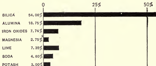
FIG. 11.—Diagram showing the chemical composition of a syenite. (After Daly, Canadian Geological Survey.)
