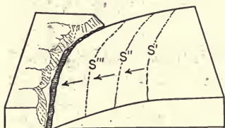
FIG. 114.—To illustrate the "slipping off" of an incised meander.
