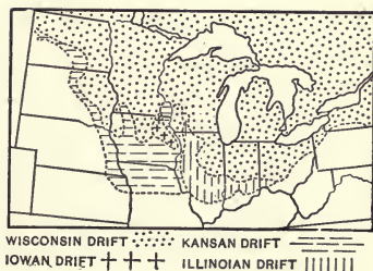
FIG. 215.—Map showing exposures of different glacial drifts. (After Leverett and Calvin.)
