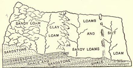
FIG. 78.—Residual soils from sedimentary rocks, Kansas. (Data after U. S. Bureau of Soils.)
