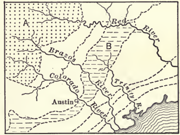
FIG. 141.—The Red, Brazos and Colorado rivers rise in regions of red Permian rocks (A). The Trinity River rises in a belt of chalks and marls (B) which furnish calcareous materials to this river.
