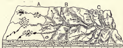
FIG. 217.—Diagram to illustrate the topography and drainage on new drift (A), old drift (B), and an unglaciated area (C).
