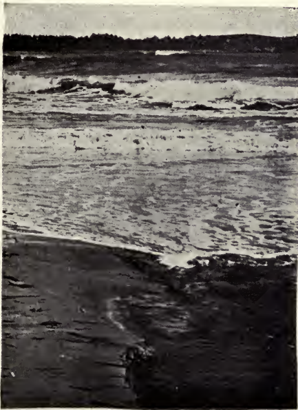
FIG. 244.—Ocean surf, Canada. (Canadian Geological Survey.)
