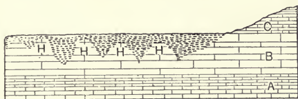
FIG. 258.—Diagram showing the occurrence of brown phosphate in Tennessee. (After Hayes, U. S. Geological Survey.)
