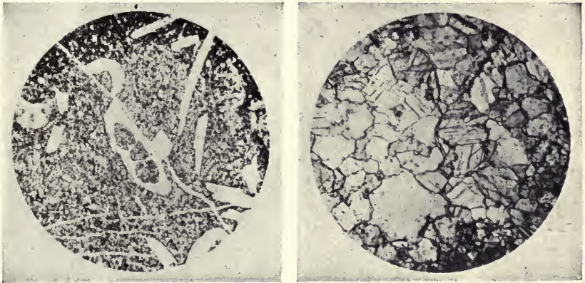
FIG. 47.—The limestone on the left has been changed to the marble on the right. Microphotograph. (U. S. Geological Survey.)
