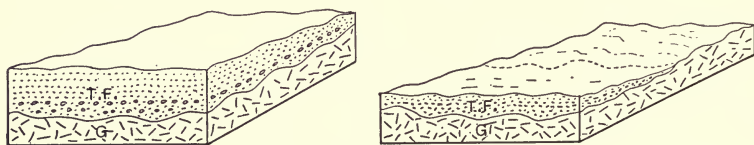
FIG. 85.—The diagram to the left shows the Tishomingo formation ( TF ) overlying granite ( G ). In the right-hand diagram, the Tishomingo formation has been mostly eroded with the result that inherited soils cover the upper part of the diagram, Okla. (Data from U. S. Geological Survey and U. S. Bureau of Soils.)
