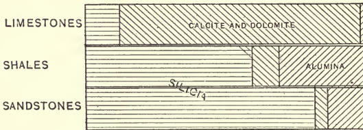
FIG. 77.—Generalized diagram to show the composition of limestones, shales and sandstones. (Data after Clarke, U. S. Geological Survey.)
