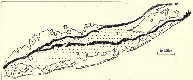
FIG. 198.—Sketch map of Long Island, N. Y., showing the two terminal moraines (1 and 2) and the two outwash plains (3 and 4). The rectangle in the western part indicates the area shown in Fig. 199.
