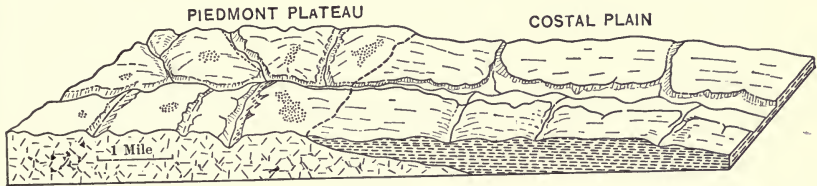
FIG. 86.—Diagram of the junction of the Coastal Plain and Piedmont Plateau. The dotted line shows the junction. The dotted areas indicate formerly overlying Coastal Plain materials which have not been entirely eroded. (Adapted from U. S. Geological Survey.)
