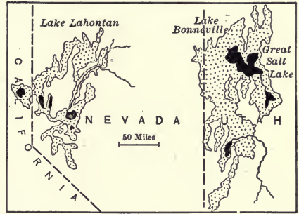
FIG. 233.—Areas formerly covered by the extinct Lakes Bonneville and Lahontan in the Great Basin. Great Salt Lake is a remnant of Lake Bonneville.
