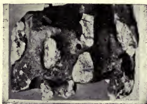
FIG. 72.—Weathering of cherty dolomitic limestone. The white portions (chert) are less weathered and project. (Mo. Geological Survey.)
