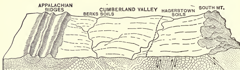
FIG. 55.—Diagram to show rock structure and topography of the Cumberland Valley and South Mt. in Pennsylvania. (Data after U. S. Geological Survey and U. S. Bureau of Soils.)
