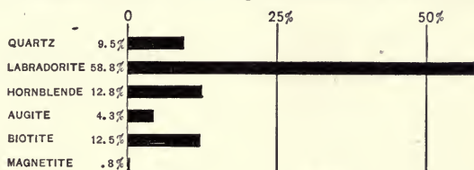
FIG. 14.—Mineralogical composition of a diorite, the chemical composition of which is shown in Fig. 13. (After Daly, Canadian Geological Survey.)
