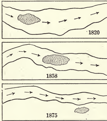
FIG. 121.—Diagram to show the downstream movement of an alluvial island (dotted), Mo.
