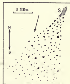
FIG. 192.—Fan-like glacial debris from outcrop ( S ). (Salisbury, N. J. Geological Survey.)
