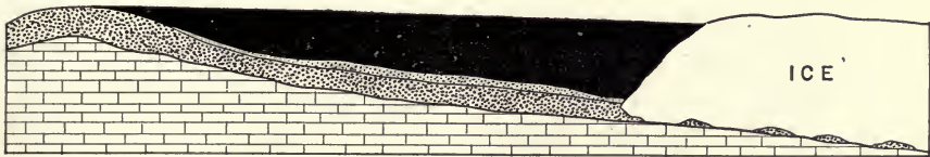
FIG. 208.—Section of a marginal glacial lake. The drainage has been blocked by ice to the right.
