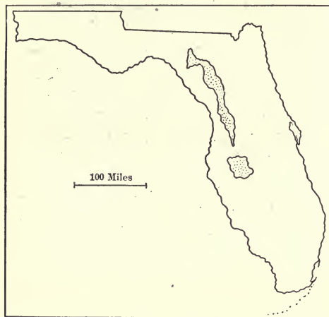
FIG. 263.—Map of Florida showing the principal phosphate areas (dotted). (Matson, U. S. Geological Survey.)
