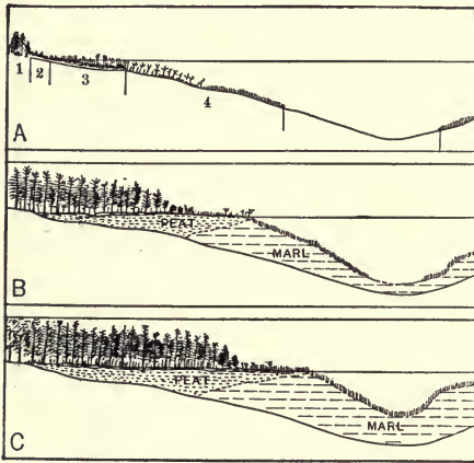
FIG. 242.—Diagram to illustrate the accumulation of peat and marl in a filling lake or swamp. A represents an early stage with the following plant zones: (1) conifers; (2) bog shrub; (3) bog hedge; (4) aquatic plants. (After Transeau.)
