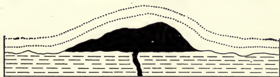
FIG. 22.—Sundance Mountain, Wyo., a laccolithic mountain (Upper photo). The sides of the mountain are partly buried in waste. The diagram below shows a mass of lava (black) which was intruded beneath overlying rock and arched it upwards. The overlying sedimentary rocks have been eroded so that the intruded lava now forms the mountain. (After Darton, U. S. Geological Survey.)
