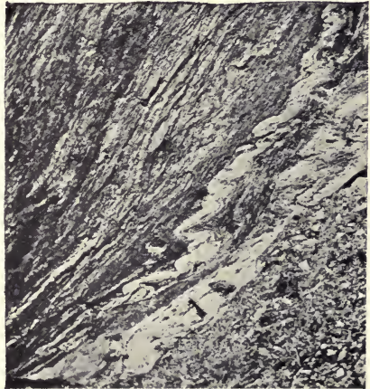
FIG. 40.—Foliated gneiss produced by intense folding. N. C. (U. S. Geological Survey.)
