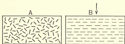
FIG. 41.—Diagram to illustrate the development of schistosity by pressure.
