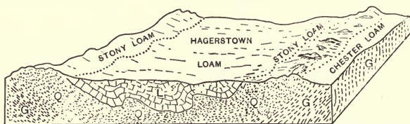
FIG. 75.—Diagram to show the occurrence of rocks and their derived soils on the Piedmont in Pennsylvania. The rocks are closely folded and include gneiss ( G ), quartzite ( Q ) and limestone ( L ). Length of section about seven miles. (Data from U. S. Bureau of Soils and U. S. Geological Survey.)
