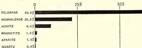
FIG. 12.—Diagram showing the mineralogical composition of a syenite, the chemical composition of which is shown in Fig. 11.
