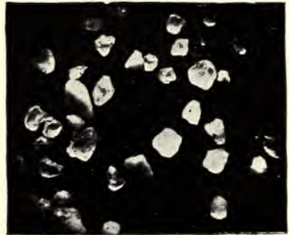
FIG. 119.—Fine river sediments. On the left are grains of rounded sand, magnified; the grains are about \frac{1}{25} of an inch in diameter. On the right are minute grains of silt, much magnified; the grains are about \frac{1}{500} of an inch in diameter. The smaller grains are much less abraded than the larger grains.
