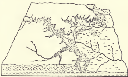
FIG. 110.—Head erosion of several streams producing an escarpment, Texas. (Data after Gould, U. S. Geological Survey.)
