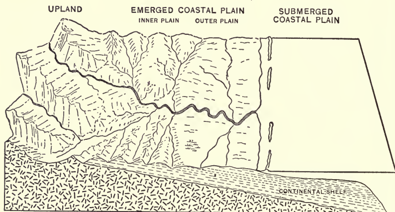
FIG. 250.—The submerged coastal plain and the inner and outer parts of the emerged coastal plain
