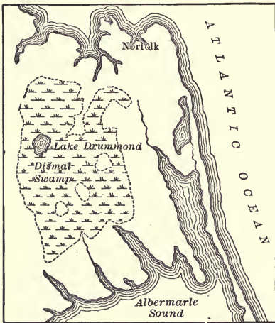
FIG. 237.—Map of Dismal Swamp, Va.
