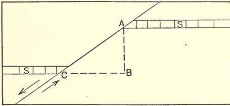
FIG. 61.—Diagram to illustrate a fault.
