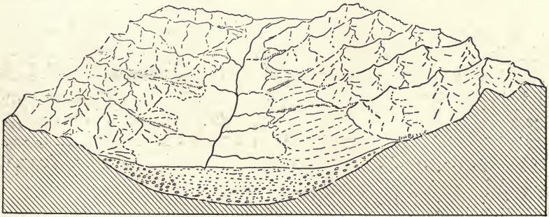
FIG. 152.—Diagram to show simple and coalesced alluvial fans. The mountains on the right are higher and the streams have built the larger alluvial fans which have grown together to form a piedmont plain.
