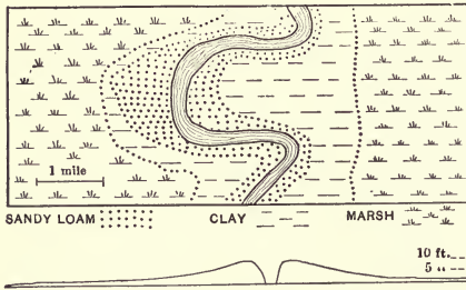
FIG. 122.—Map of a portion of the Mississippi flood plain (above). Below is a profile taken across the center of the map. (Data from U. S. Bureau of Soils.)
