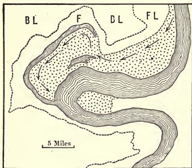
FIG. 134.—Showing the deposition of soils (dotted areas) as a meander of the Mississippi moves down stream. The arrows indicate approximately the former position of the river, Louisiana. ( FL ) front land; ( BL ) back land.
