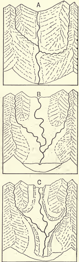
FIG. 139.—Diagram to illustrate (A) valley cutting; (B) valley filling; (C) terrace making.
