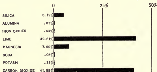
FIG. 37.—Composite analysis of 345 limestones. (After H. N. Stokes, U. S. Geological Survey.)
