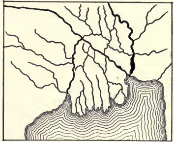
FIG. 146.—Combined delta of the Brahmaputra and Ganges rivers. (After Geikie.)
