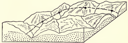
FIG. 99.—Diagram to show a common relation between topography and ground water (dotted). Springs (S) occur where the water table is reached in valleys.
