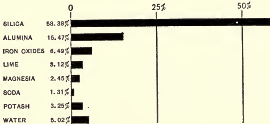
FIG. 33.—Composite analysis of 78 shales. (After Stokes, U. S. Geological Survey.)
