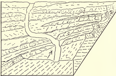
FIG. 58.—Ridges caused by folding. Distant view above; the first ridge is Blue Mountain. The Diagram below shows four ridges made by sandstones (S) which have been upturned by folding. The arrow shows the position of the camera. The two ridges in the foreground of the diagram are those shown in the photograph. Penna.
