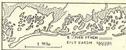
FIG. 246.—Barrier beaches and partly filled lagoons on Long Island, N. Y. (U. S. Bureau of Soils.)
