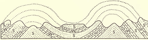
FIG. 57.—Diagram to illustrate the development of ridges and valleys on folded rocks. The strong rocks (S) make the ridges and the weak rocks (W), the valleys. The dotted lines indicate the eroded strata.
