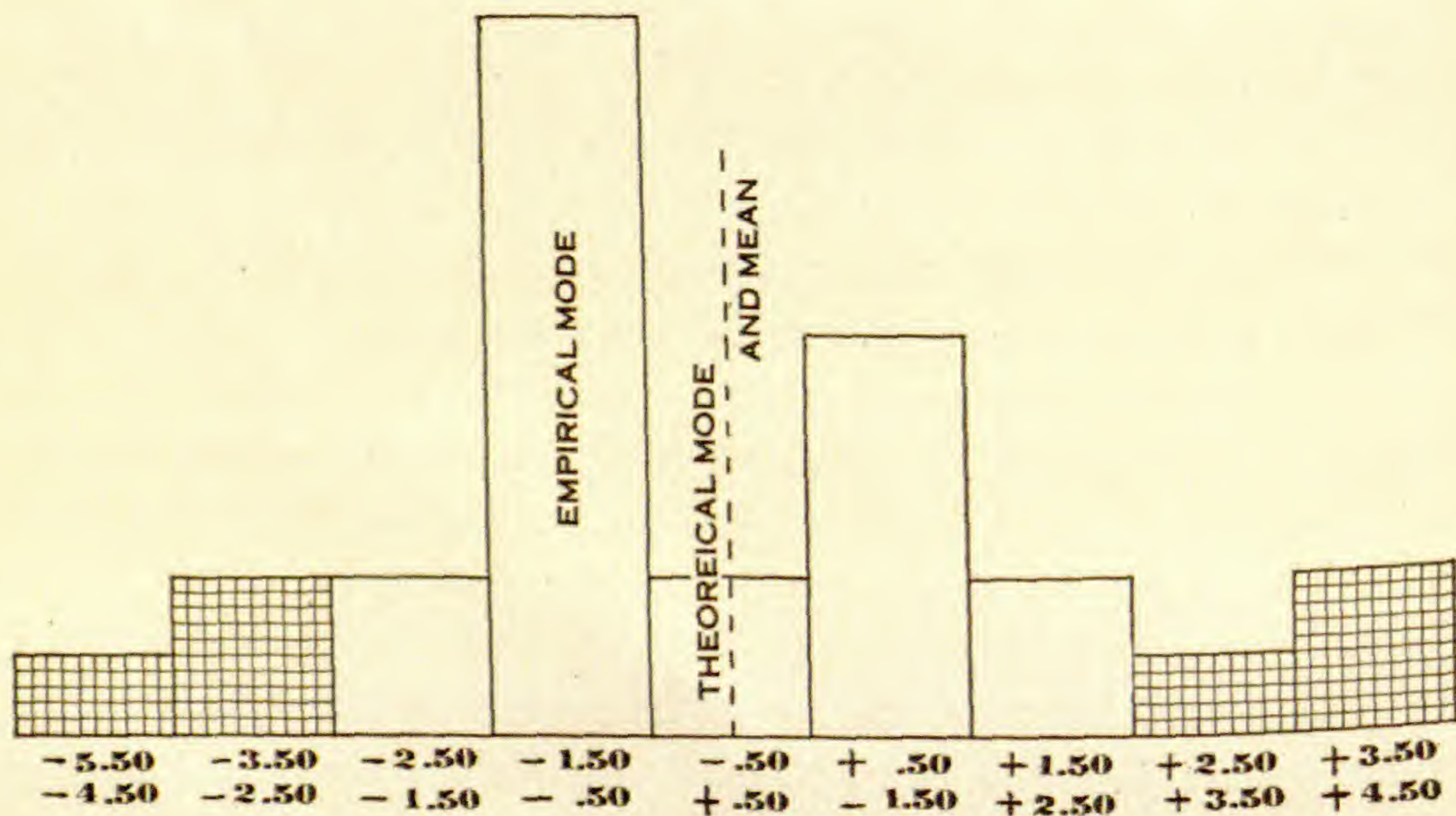
FIG. 4. Distribution of ratios of r_{oz} to E_{r_{oz}} , Ohio series.
