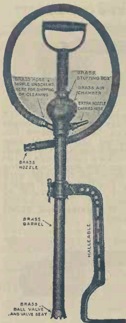
No. 32 Bucket Pump.
