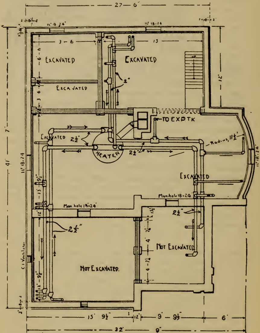
FOUNDATION PLAN. Ceiling 6'.
