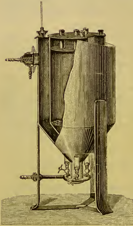
FIG. 16.—D'ARSONVAL'S INCUBATOR.
