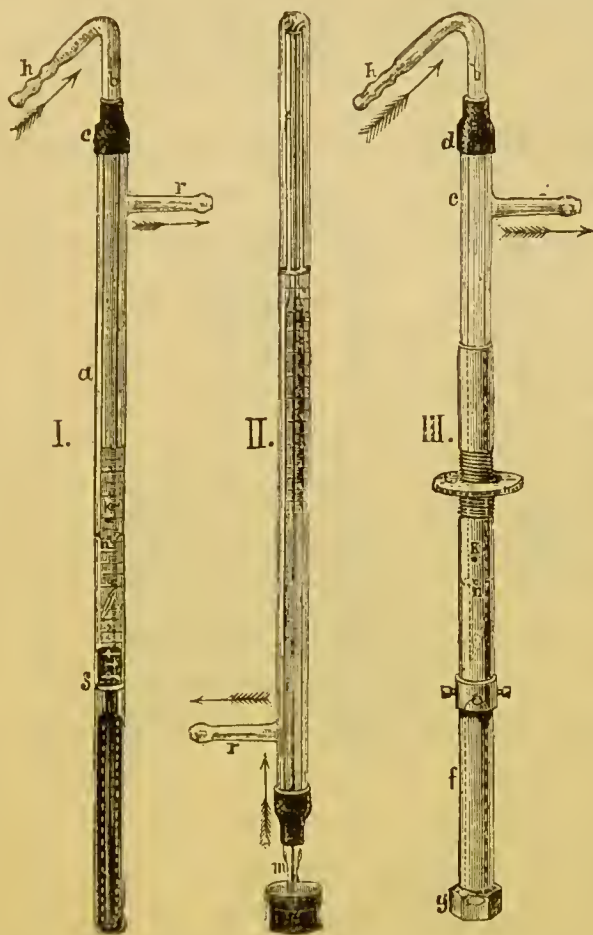
FIG. 23.—MEYER'S THERMO-REGULATOR.
