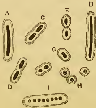
FIG. 77.— BACTERIUM PNEUMONIÆ CROUPOSÆ , FROM PLEURAL CAVITY OF A MOUSE, \times 1500 . A, B. Thread-forms. C, D, E. Short rod-forms. G. Diplococci. H. Cocci. I. Streptococci. [After Zopf.]
