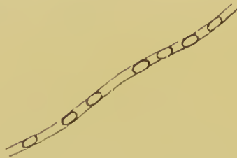
FIG. 111.—SPORES OF BACILLUS ANTHRACIS UNSTAINED, \times 1500 .
