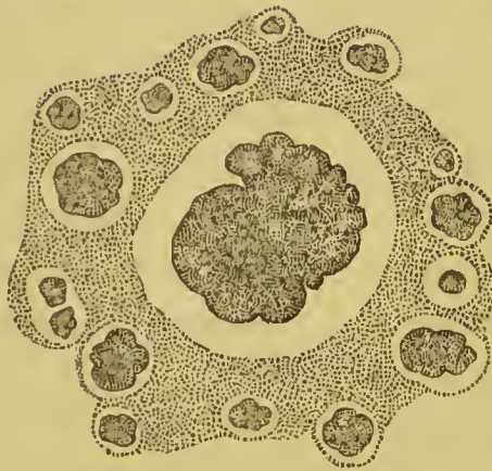
FIG. 47.—ASCOCOCCUS BILLROTHII, \times 65 . [After Cohn.]
