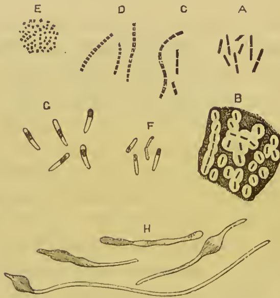
FIG. 120. BACILLUS CYANOGENUS , \times 650 .
