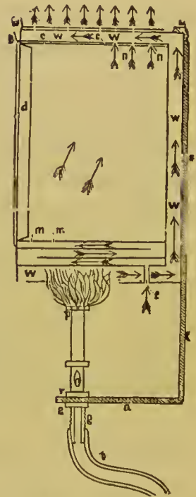
FIG. 3.—SECTION OF HOT-AIR STERILISER.
