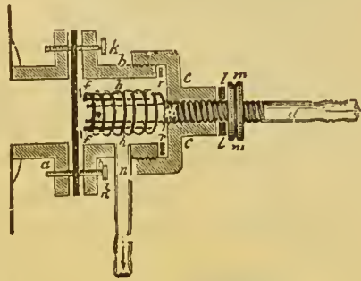
FIG. 17.—SCHLOSING'S MEMBRANE REGULATOR.
