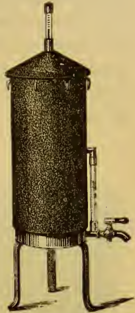
FIG. 1.—KOCH'S STEAM-STERILISER.
