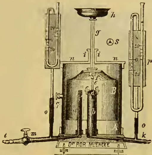
FIG. 19. MOITESSIER'S GAS-PRESSURE REGULATOR.
