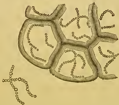
FIG. 56.— LEUCONOSTOC MESENEROIDES ; COCCI-CHAINS WITH ARTHROSPORES (after Van Tieghem and Cienkowski).
