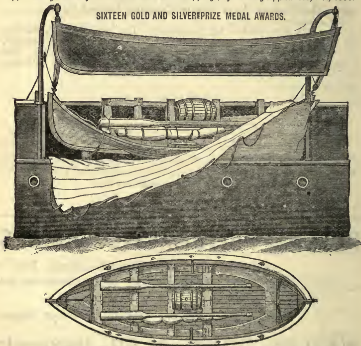
Berthon Ship's Boat folded on davits, and plan of one ready for use.
