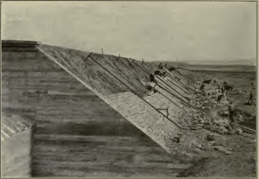
FIG. C.—Paving on water side of earth embankment. Belle Fourche River, So. Dak.
