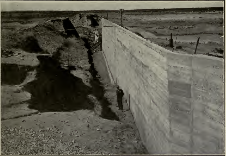
FIG. A.—Concrete core wall in earth dam. Carlsbad Project, N. Mex.
