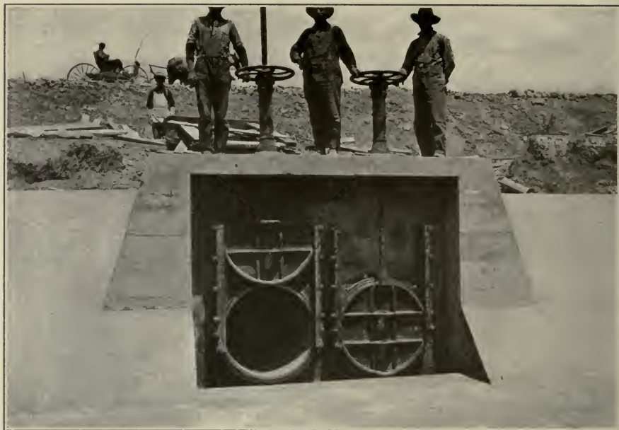
FIG. C.—Cast-iron valves on distributing systems instead of the usual wooden gates. Uncompahgre Project, Colo.
