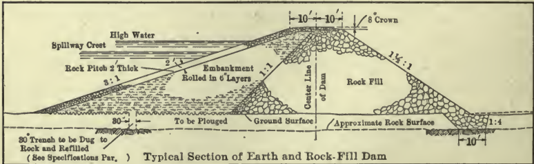
FIG. 46.—Typical section of earth and rock-fill dam, Clear Lake dam, Klamath Project, Oregon.
