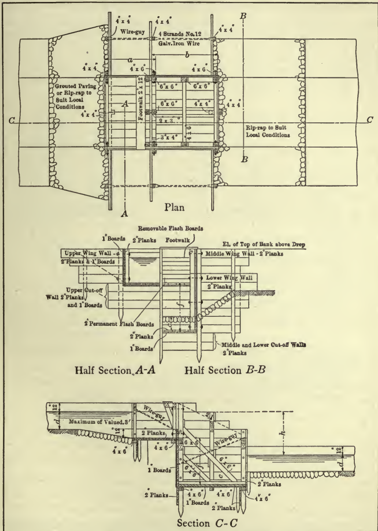
FIG. 22.—Type of timber drop for small canals.
