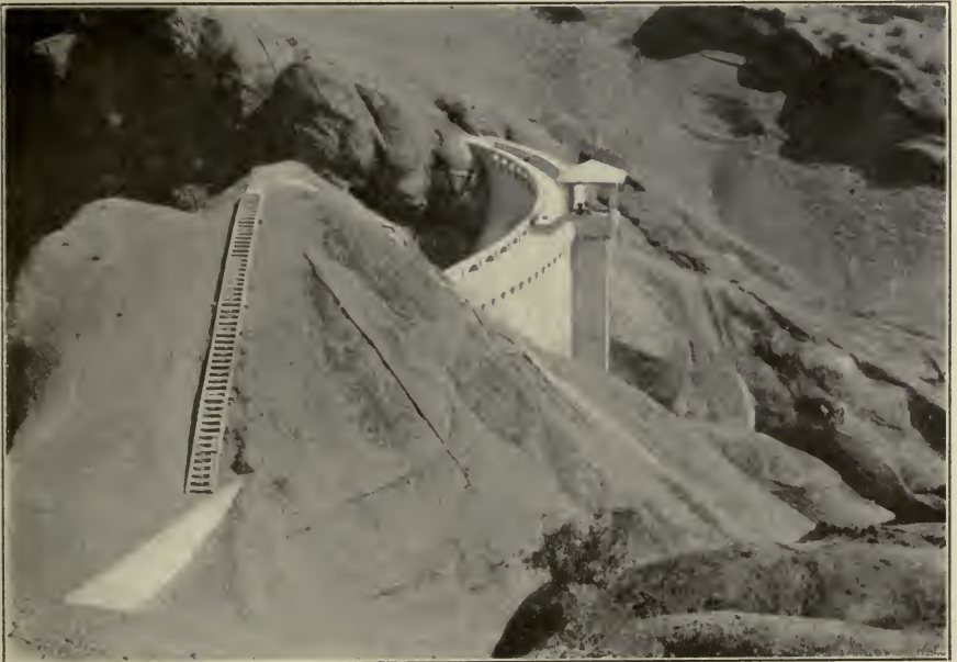
FIG. B.—Concrete structure for regulating floods. East Park dam, Orland Project, Cal.
