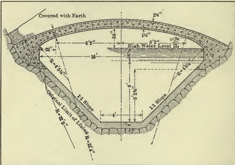
FIG. 13.—Cement lined canal with reinforced concrete arch cover later added to catch the loose, sliding debris from steep hill slopes, Strawberry Valley Project, Utah.
