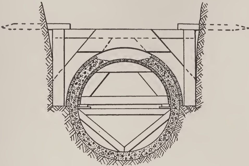
FIG. 26.—FORM FOR CONCRETE ARCH.
