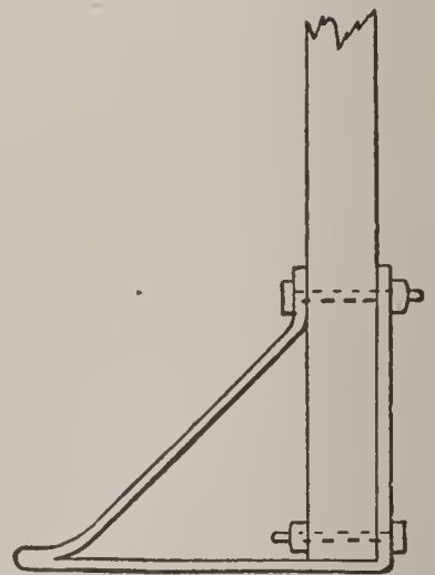
FIG. 8.—GRADE-ROD.
