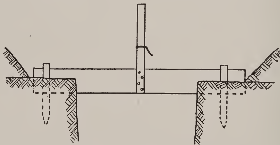
FIG. 5.—METHOD OF SETTING GRADE-PLANK.
