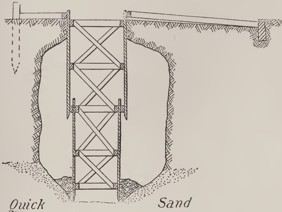
FIG. 28.—SHEATHING A BADLY CAVED TRENCH.
