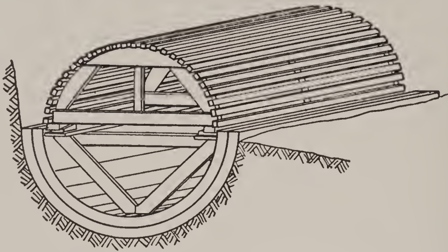
FIG. 25.—CENTRE FOR BRICK SEWERS.
