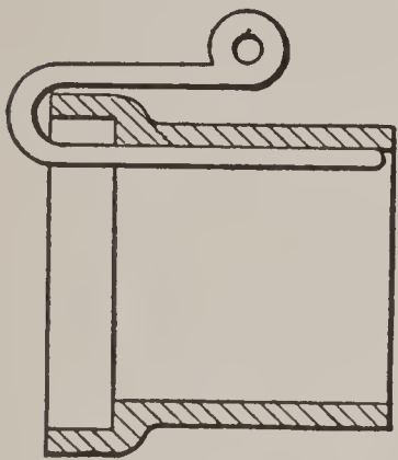
FIG. 19.—PIPE-LAYING HOOK.
