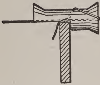
FIG. 7.—METHOD OF HOLDING GRADE-CORD.
