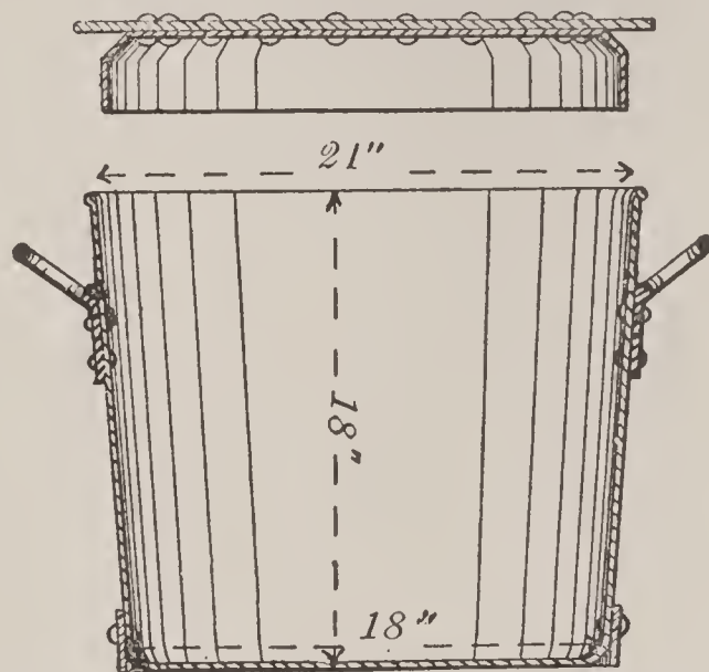
FIG. I.—MODIFIED BIRMINGHAM PAIL.
