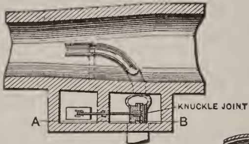
FIG. 2. INTERCEPTOR (DIVERTING).
