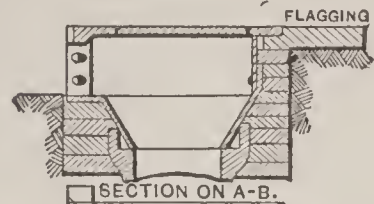
FIG. 5. STONE TOP INLET WITH CATCH-BASIN.
