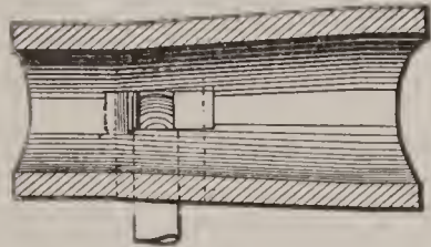
FIG. 1. INTERCEPTOR (LEAPING WEIR).
