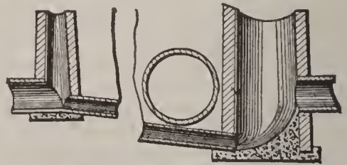
FIG. 6. INVERTED SIPHON.
