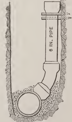
FIG. 7. DEEP-CUT 'HOUSE CONNECTION.
