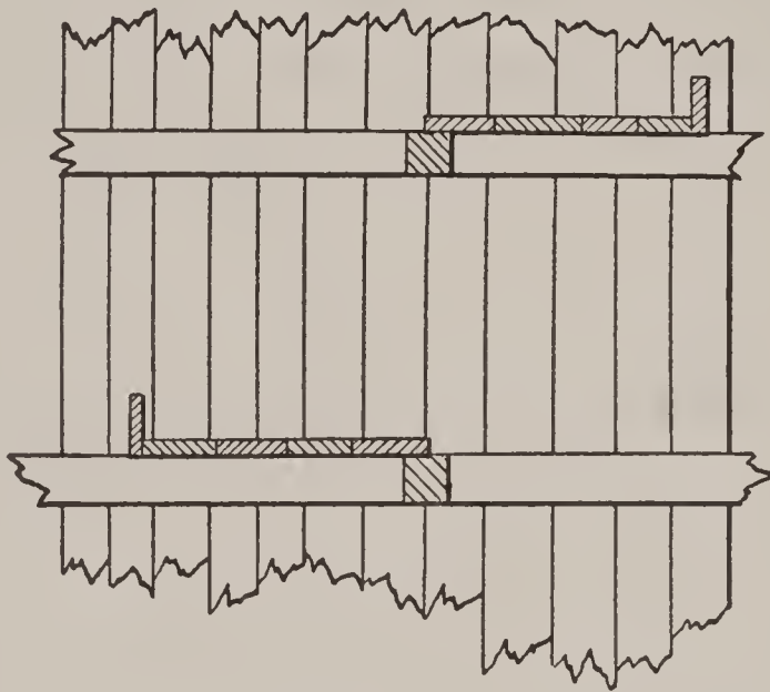
FIG. 12.—CROSS-STAGING IN TRENCH.
