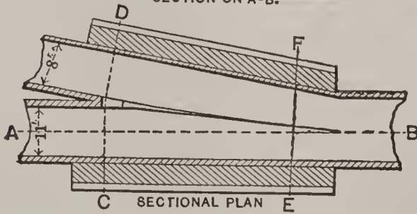
FIG. 6. JUNCTION OF 8 FT. AND 11 FT. SEWERS.
