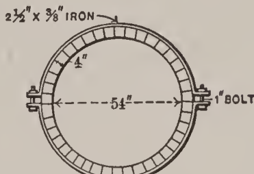
FIG. 4. WOODEN OUTLET SEWER NEW YORK CITY.
