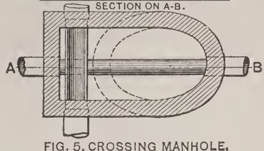
FIG. 5. CROSSING MANHOLE.
