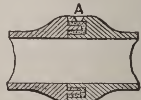
FIG. 11. "ARCHER" JOINT.
