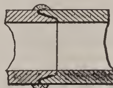
FIG. 10. BEVEL JOINT.
