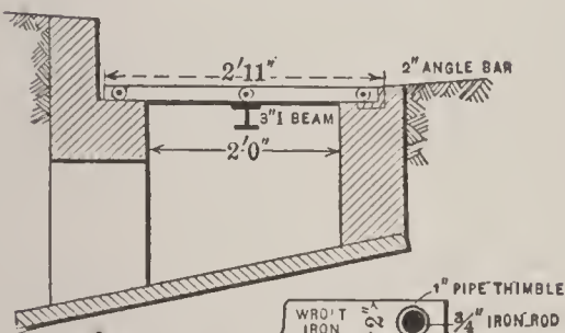
FIG. 1. FLUSHTANK
