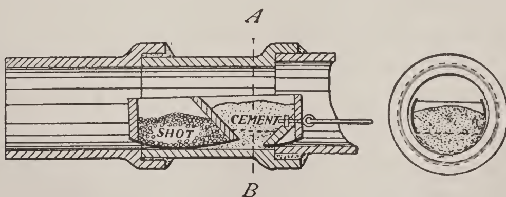
FIG. 10.—INVERT-FORMER.
