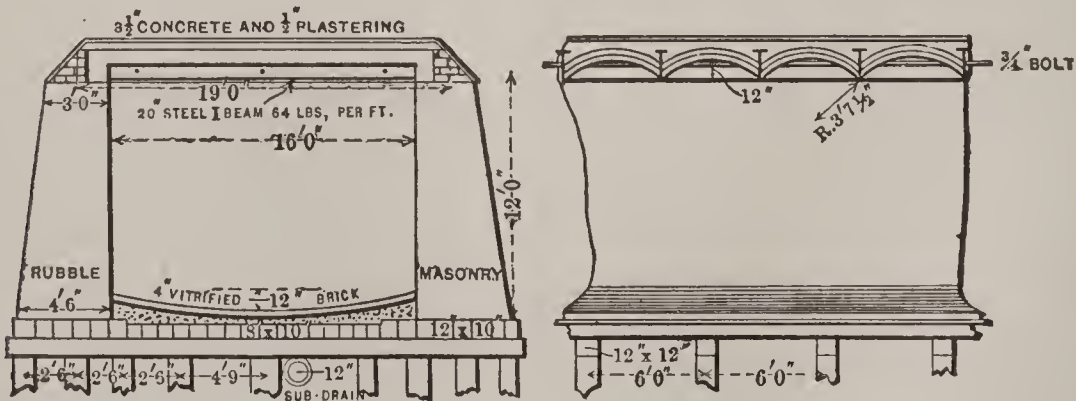
FIG. 10. CANAL STREET SEWER; ST. PAUL, MINN.
