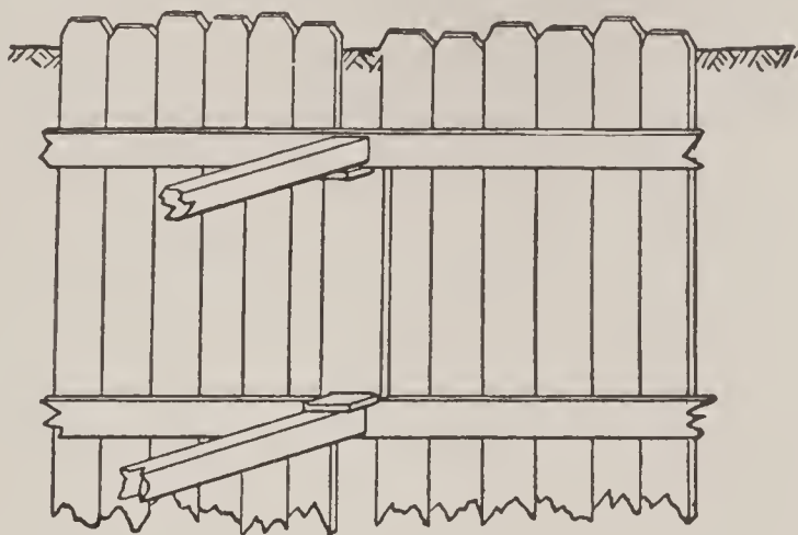
FIG. 14.—SHEATHING UNDER BRACES.
