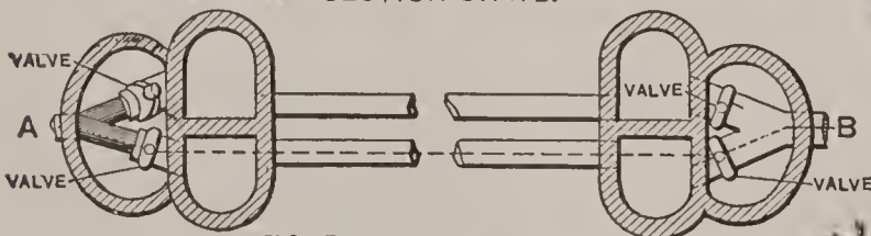
FIG. 5. INVERTED SIPHON.
