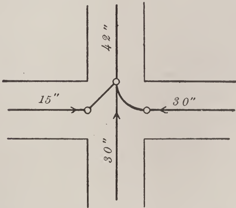
FIG. 4.—ALIGNMENT OF SEWER-JUNCTIONS.
