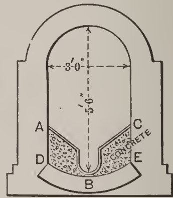
FIG. 7. OLD LONDON SEWER WITH IMPROVED INVERT.
