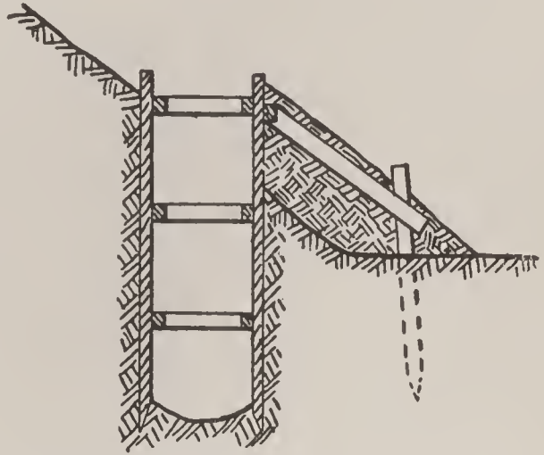
FIG. 32.—SHEATHING ON STEEP SLOPES.
