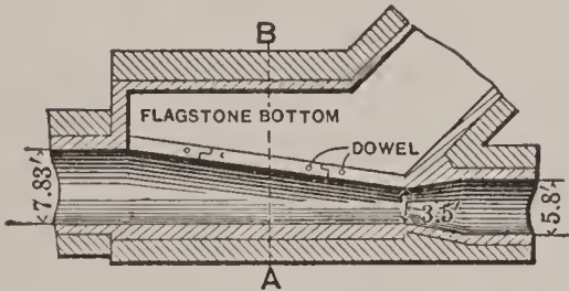
FIG. 3. STORM OVERFLOW, DENVER, COLO.
