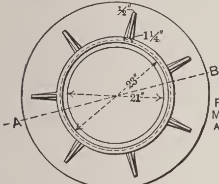
FIG. 7. BROOKLYN MANHOLE TOP.
