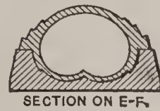
FIG. 6. JUNCTION OF 8 FT. AND 11 FT. SEWERS.
