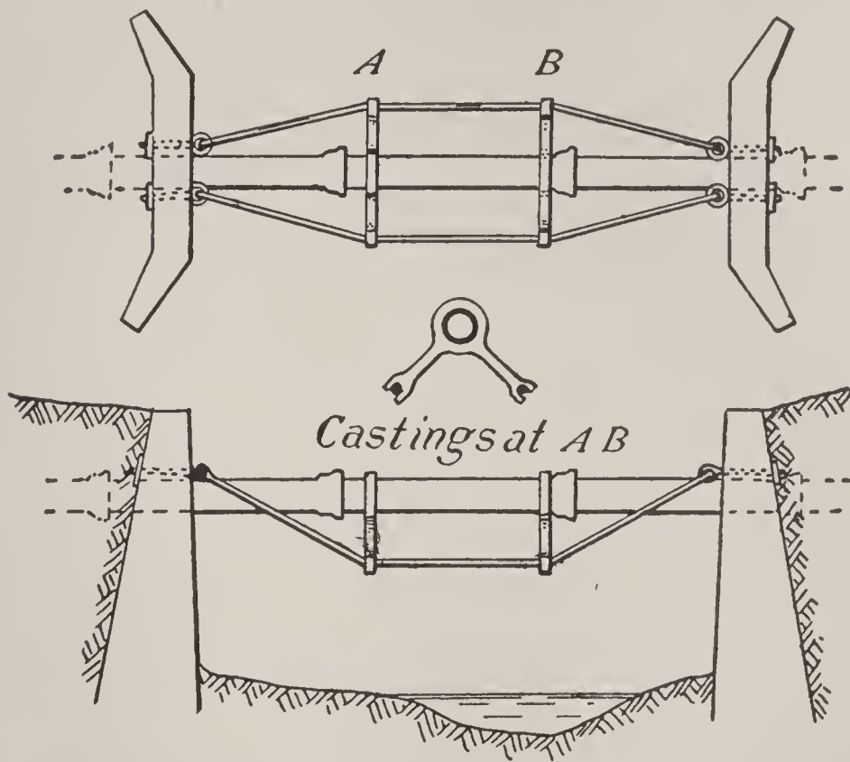
FIG. 30.—SEWER CROSSING CREEK ABOVE WATER.
