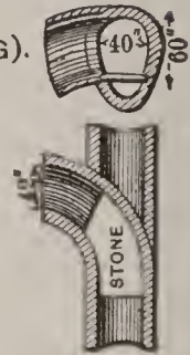
FIG. 4. BROOKLYN OVERFLOW.
