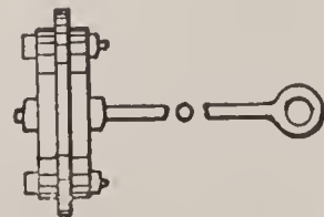
FIG. 21.—PIPE-CLEANING DISK.
