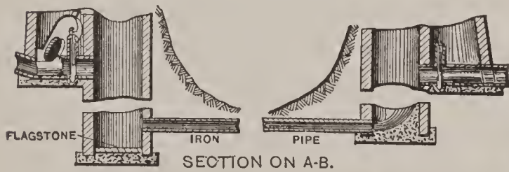
FIG. 3. STORM OVERFLOW, DENVER, COLO.
