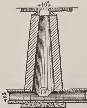
FIG. 11. BRICK LAMPHOLE.
