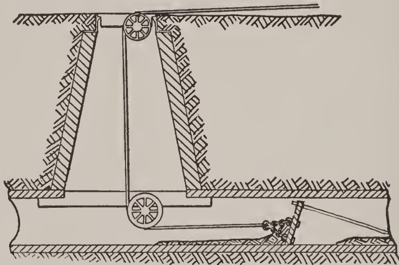
FIG. 36.—METHOD OF USING CLEANING-DISK.
