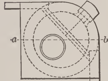
FIG. 5. STONE TOP INLET WITH CATCH-BASIN.
