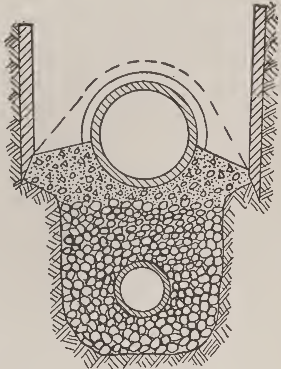
FIG. 27.—SEWER-PIPE LAID IN CONCRETE.
