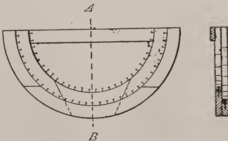
FIG. 22.—TEMPLET FOR BRICK SEWERS.
