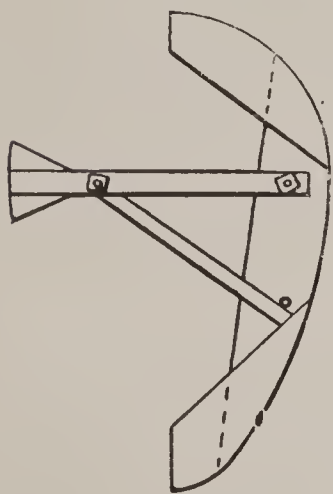
FIG. 9.—INSPECTOR'S TEMPLET FOR EGG- SHAPED SEWER.
