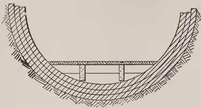
FIG. 24.—MASONS' PLATFORM FOR BRICK SEWERS.
