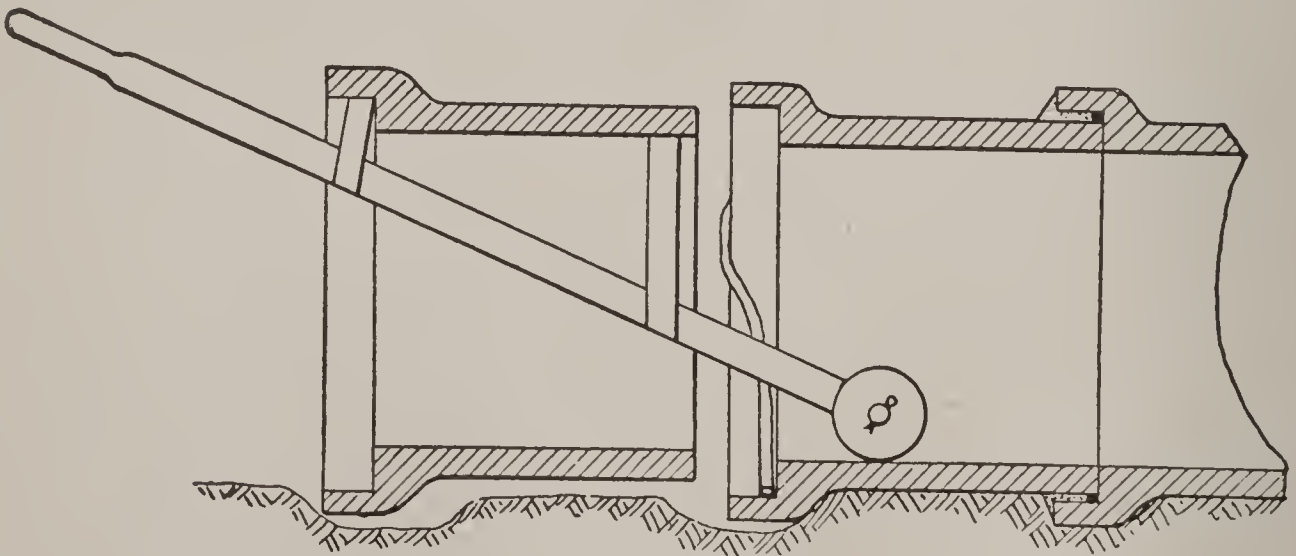
FIG. 20.—APPLIANCE FOR "ENTERING" HEAVY PIPE.
