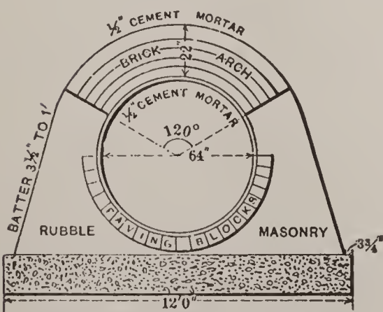
SPECIAL SECTION BENEATH RAILWAYS
