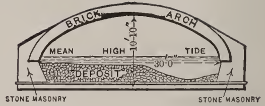
FIG. 4. TIBER CREEK, (WASHINGTON) SEWER IN 1893.
