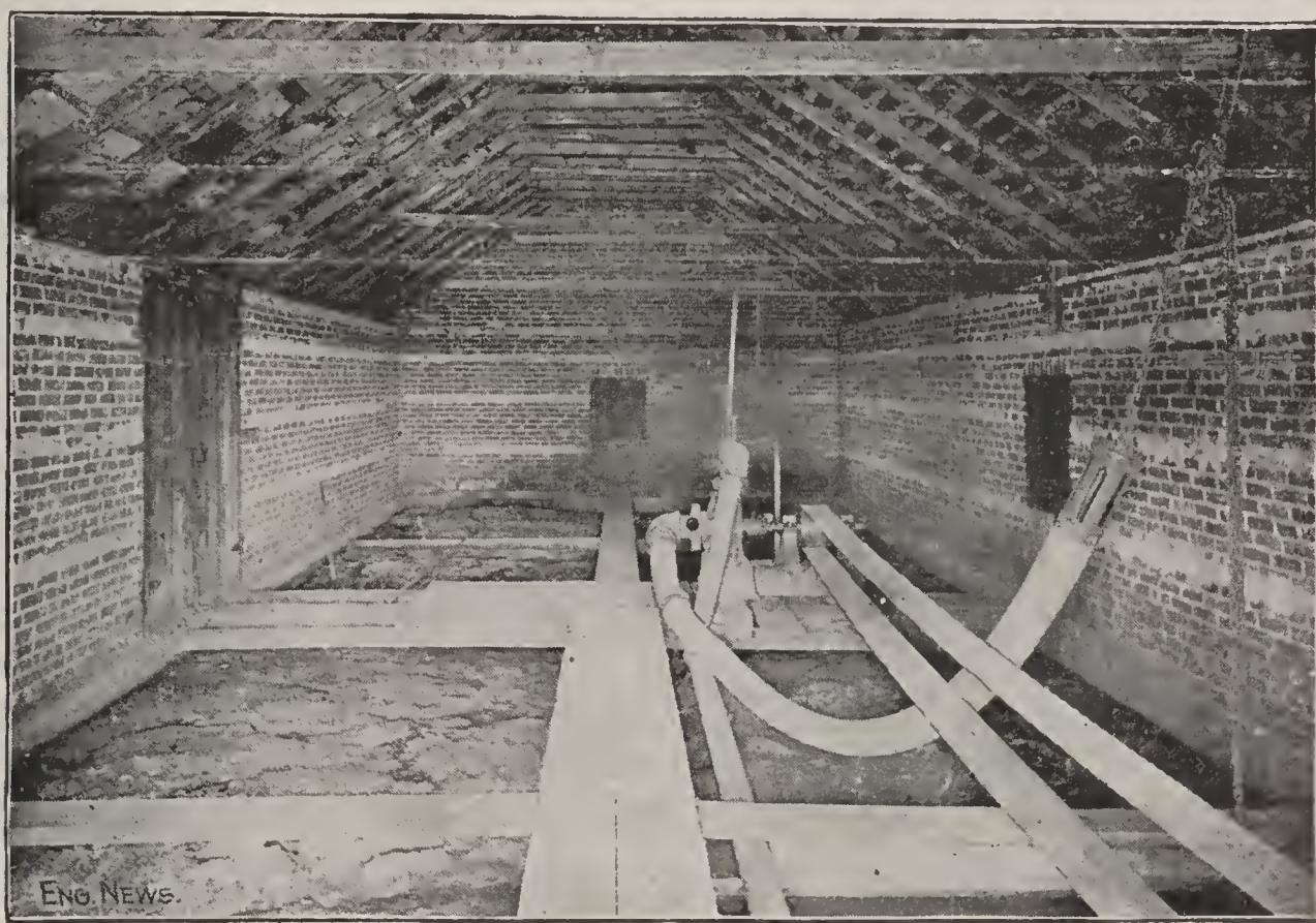
FIG. 38—INTERIOR OF CHAMPAIGN, ILL., SEPTIC TANK.
