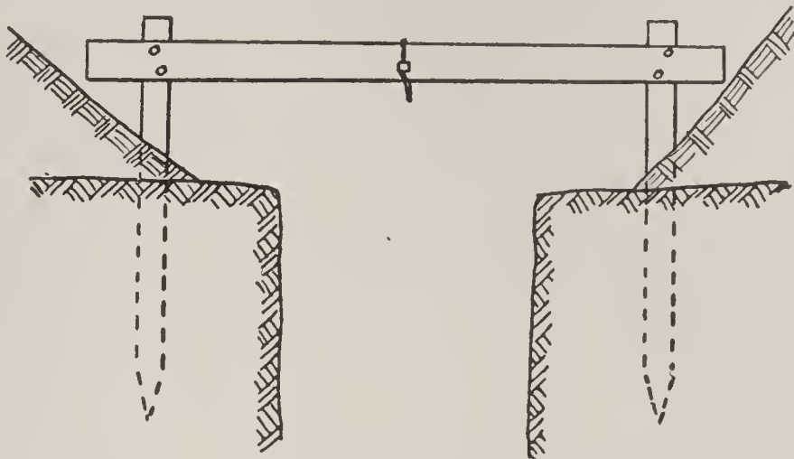
FIG. 6.—METHOD OF SETTING GRADE-PLANK.
