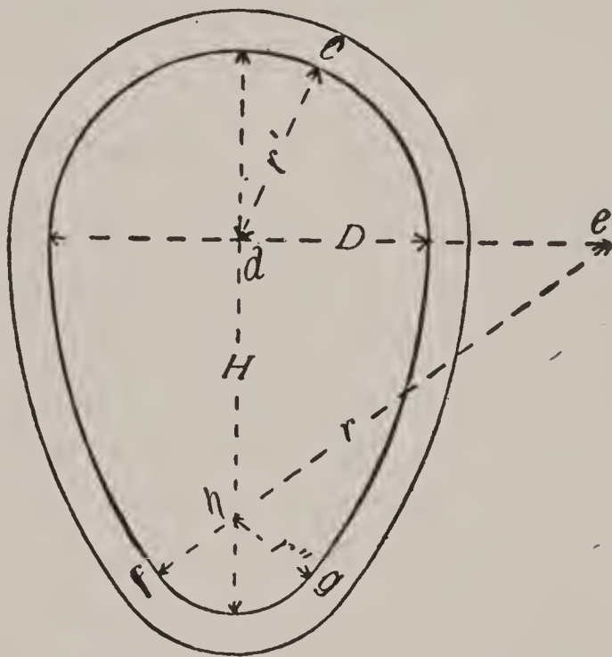
FIG. 2.—EGG-SHAPED SEWER.
