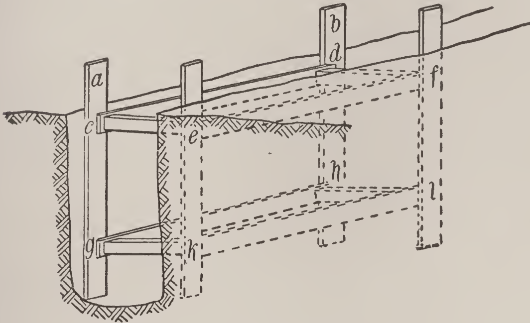
FIG. 13.—SKELETON SHEATHING.
