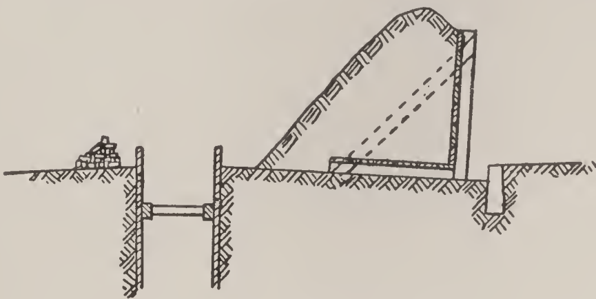
FIG. 11.—EXCAVATION-PLATFORM.
