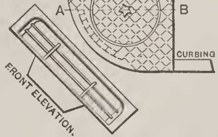
FIG. 6. IRON CURB INLET
