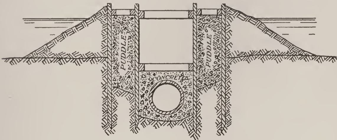
FIG. 31.—COFFER-DAM PUDDLE-WALLS.
