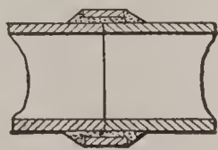
FIG. 9. RING JOINT.
