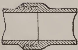
FIG. 8. HUB & SPIGOT JOINT.
