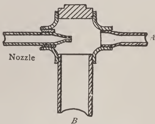
FIG. 34.—APPLIANCE FOR CLEANING SIPHON-SUMP.
