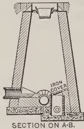
FIG. 3. GUTTER INLET COVER; BROOKLYN, 1896.
