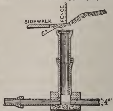
FIG. 10. HOUSE CONNECTION INSPECTION HOLE.
