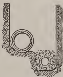
FIG. 7. SUB-DRAIN.
