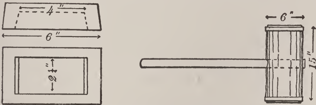
FIG. 15.—DRIVING-CAP AND MAUL.
