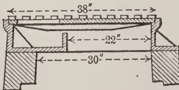
FIG. 7. BROOKLYN MANHOLE TOP.
