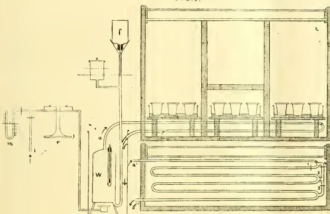
FIG. 41.—GERMINATING APPARATUS.
