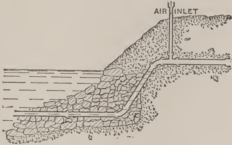
Figure 33. — Outlet of sewer, with ventilation inlet.
