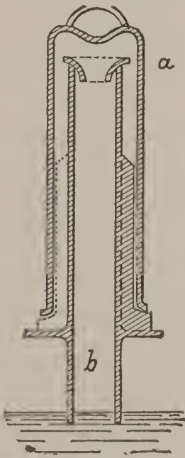
Figure 39. — Rogers Field's Annular Siphon.
