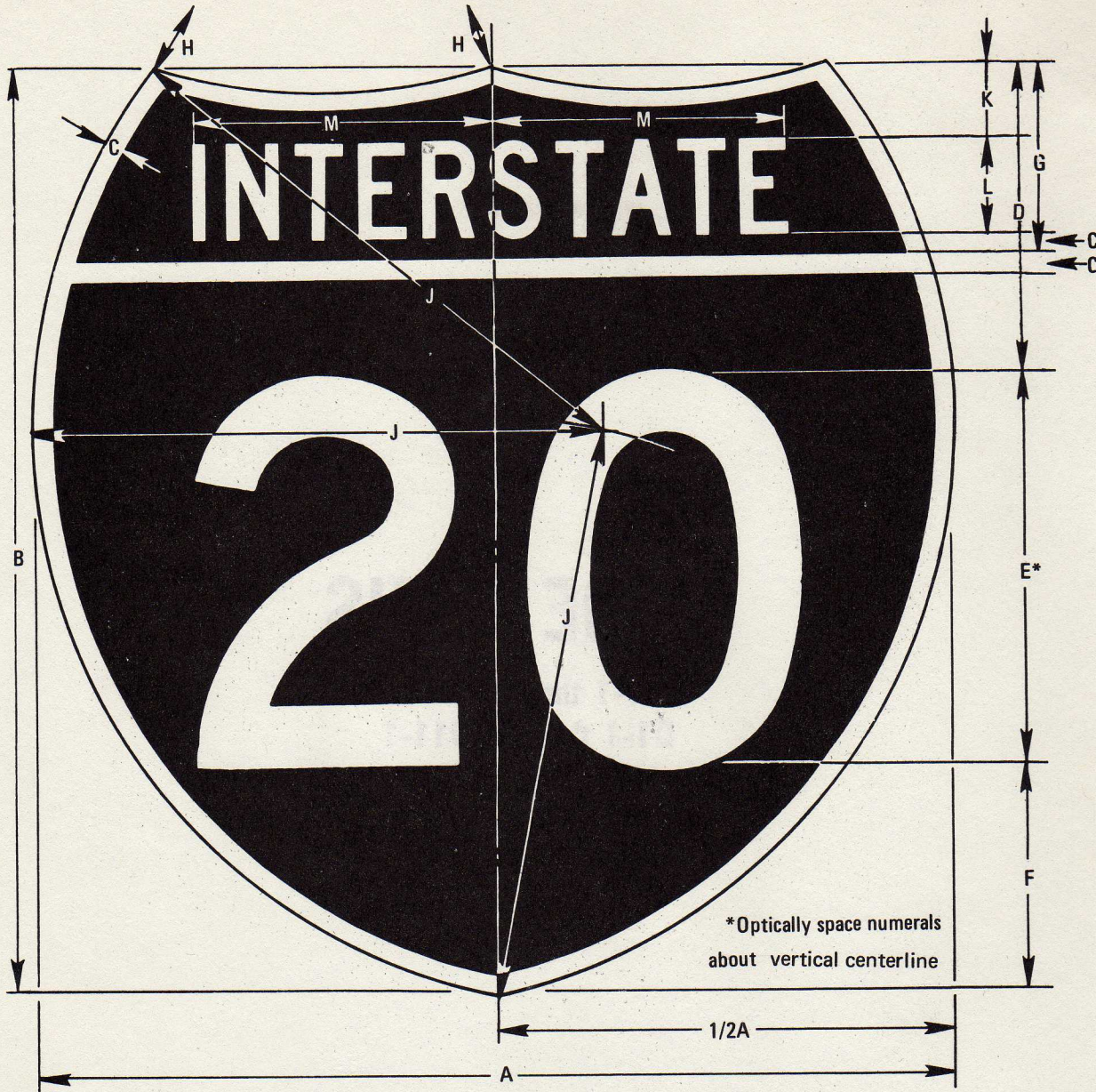
M1-1 INTERSTATE SHIELD FOR INDEPENDENT & GUIDE SIGN USE
