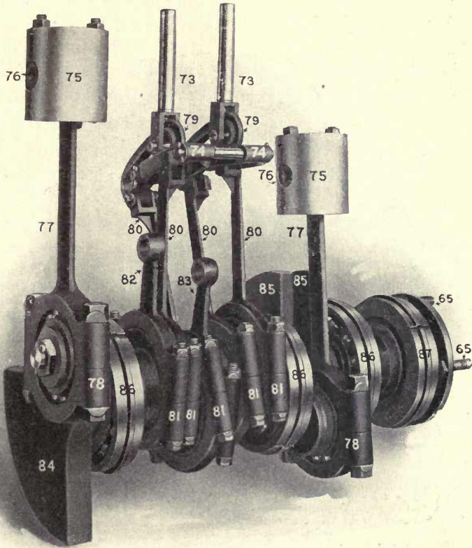
Fig. 147A. Crank-Shaft, Crank Eccentrics, and Link Motion in White Steam Car.
