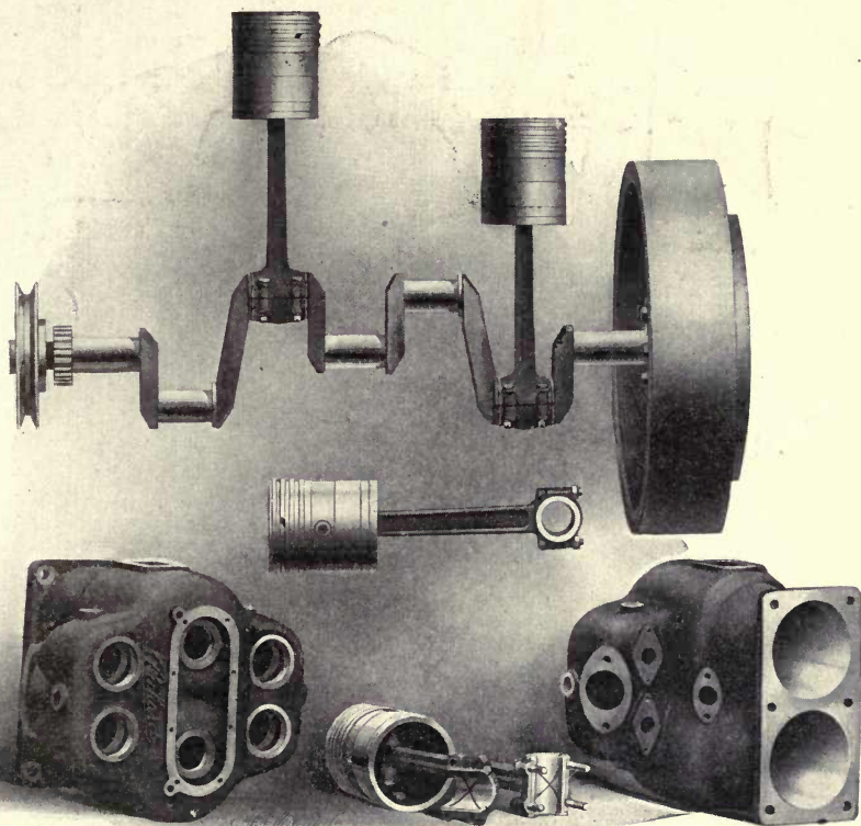
Fig. 37. Disassembled Motor of Packard Car, Showing Cylinders, Pistons, Connecting Rods, Crank-Shaft, and Fly-Wheel. Cast-in-Pair Type of Cylinder Construction. Packard Motor Car Company, Detroit, Mich.
