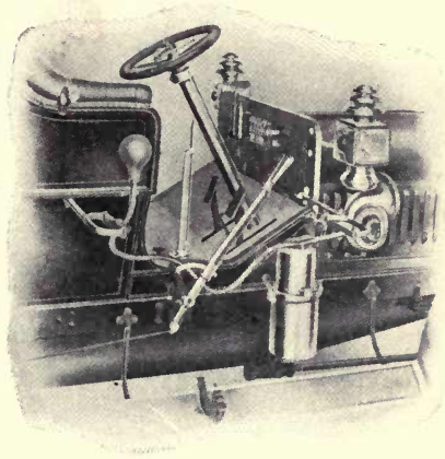
Fig. 93. Steering Column, Control Levers, and Other Operating Devices of Locomobile Car. Locomobile Company of America, Bridgeport, Conn.
