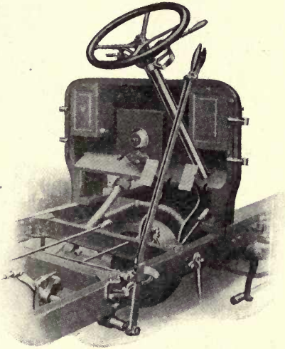
Fig. 92. Steering Column, Control Levers, and Emergency Brake of Great Arrow Car. George N. Pierce Company, Buffalo, N. Y.
