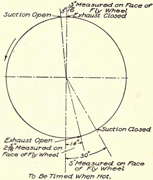
Fig. 46. Diagram Showing How to Use Fly-Wheel to Regulate the Setting of Valves for Proper Timing. The angles indicated vary with different engines, distances along circumference as indicated in inches apply to a fly-wheel 19 inches in diameter.
