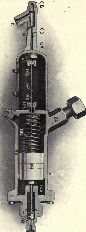
Fig. 147C. Flow Motor of White Steam Car. CB—Plug; K—Fuel Pipe to Flow Motor; L—Flow-Motor Fuel Valve; CA to CD—Graduation Valve Stem; M—Pipe to Vaporizer; AC—Stuffing-Box; 193—Valve Stem; 194—Valve-Stem Lock Nut; 192—Piston-Rod; 125—Stuffing-Box; 124—Outlet; 196—Plug for Draining; 198—Piston Spring; 191—Piston; 195—Groove; 123—Inlet; 197—By-Pass Valve.
