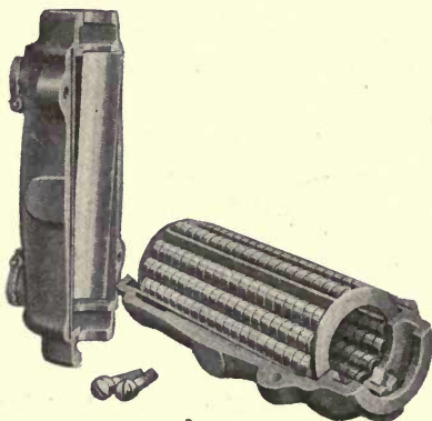
Fig. 125. Hyatt Standard Bushing Hyatt Roller Bearing Company, Harrison, N. J.
