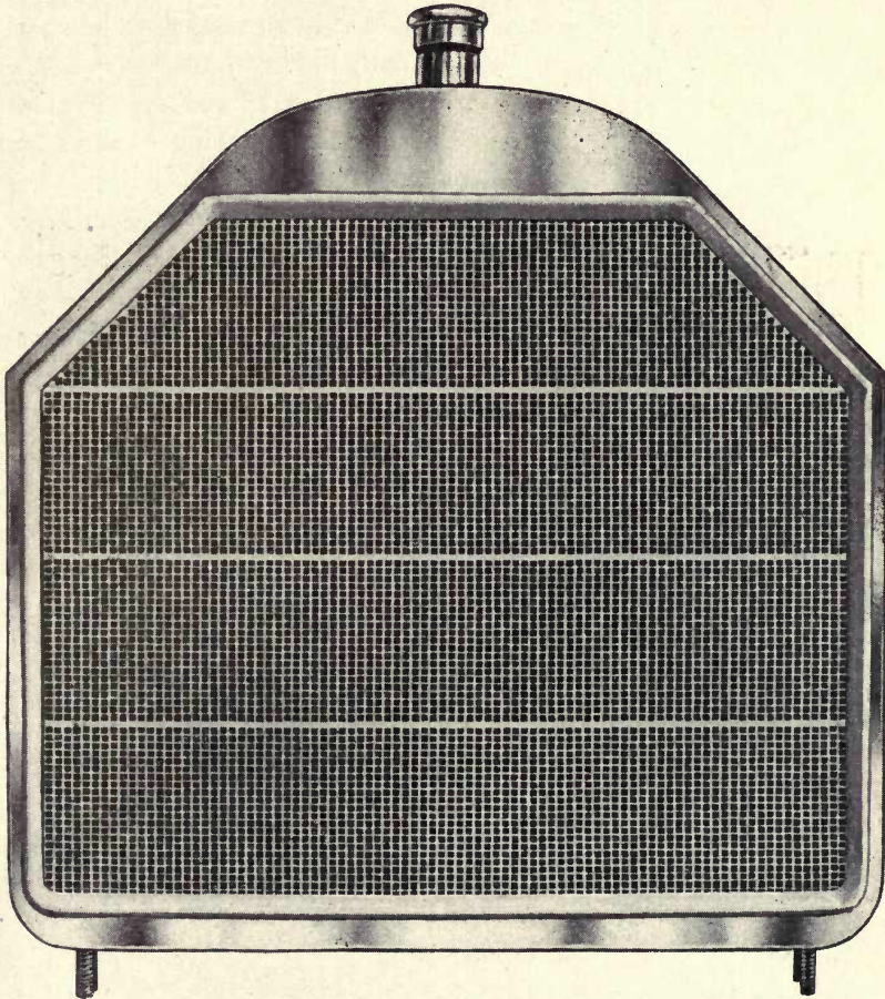
Fig. 61. Mayo Cellular Radiator of Type Used in Stearns 30-60-H. P. Cars. Mayo Radiator Company, New Haven, Conn.
