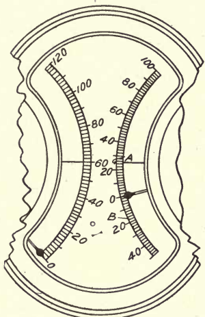
Fig. 137. Volt-Ammeter Face as Usually Graduated.
