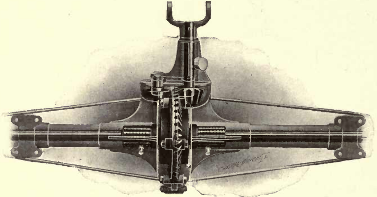
Fig. 114. Rear-Axle Construction on Maxwell Car, Showing Roller Thrust to Relieve Strain on Large Driven Bevel Gear of Differential Maxwell-Briscoe Motor Company, Tarrytown, N. Y.
