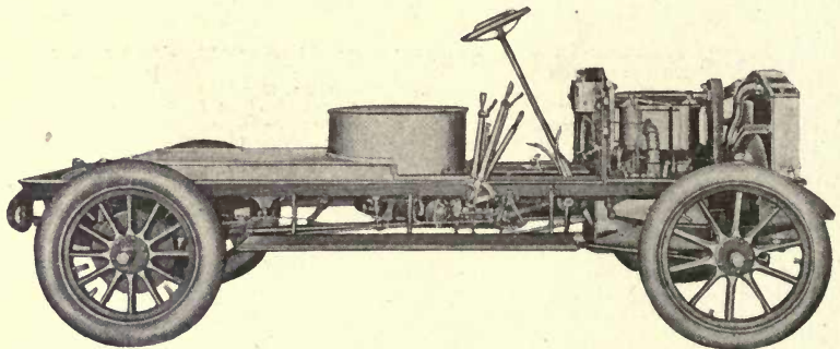
Fig. 147. Chassis of White Steamer, Showing Power Plant. The White Company, Cleveland, Ohio.
