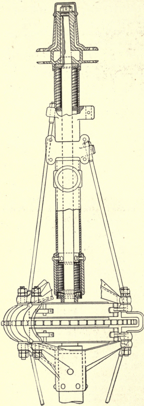
Fig. 14. Live Rear Axle, Halves Meeting at Differential. Chain-Driven, as Used in Cadillac Automobile, Detroit, Mich. Hyatt Roller Bearing Company, Harrison, N. J.
