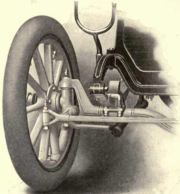
Fig. 18. Steering Yoke, Neck, and Knuckle. Packard Motor Car Company, Detroit, Mich.
