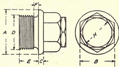
Fig. 86. Design and Dimensions of Standard Spark-Plug, Association of Licensed Automobile Manufacturers. A—1½ in.; B—¾ in.; C—¼ in.; D—¾ in.; E—Minimum, ½ in.; E'—Maximum, ⅙ in.; H—¾ in.
