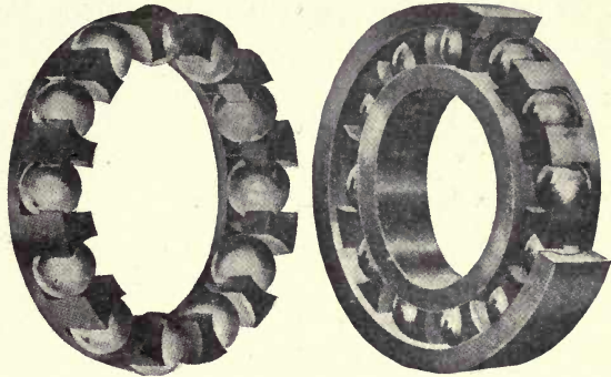
Fig. 126. Annular Ball Bearing. Silent Type with Cage Spacer. Standard Roller Bearing Company, Philadelphia, Pa.
