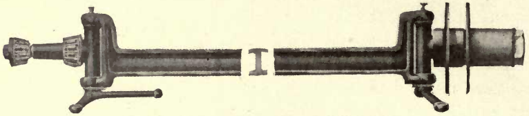
Fig. 21. Steering Arm, Showing Ball Joint. Timken Roller Bearing Axle Company, Canton, Ohio.
