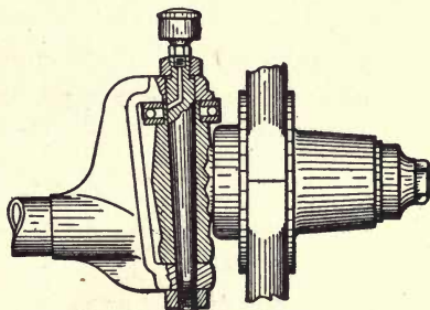
Fig. 19. Detail of Steering Knuckle, Rambler Car. Thomas B. Jeffery & Co., Kenosha, Wis.
