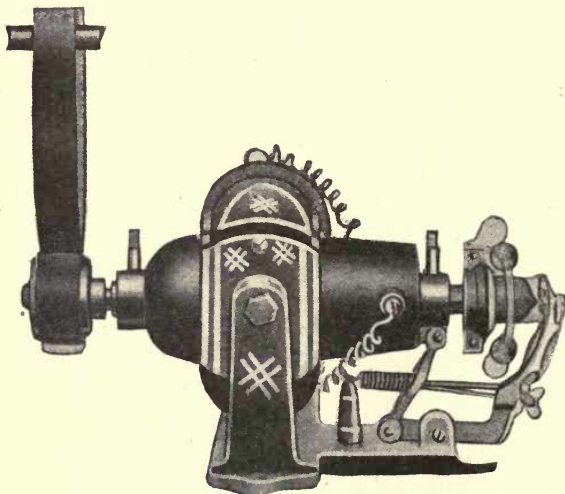
Fig. 79. Direct-Current Shunt-Wound Dynamo Driven by Gasoline Engine in Car and Used for Charging Storage Battery.
