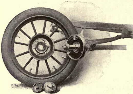
Fig. 119. Rear Wheel of Studebaker Model G Car, Showing Hub Drum and Brake. Studebaker Bros. Mfg. Co., South Bend, Ind.
