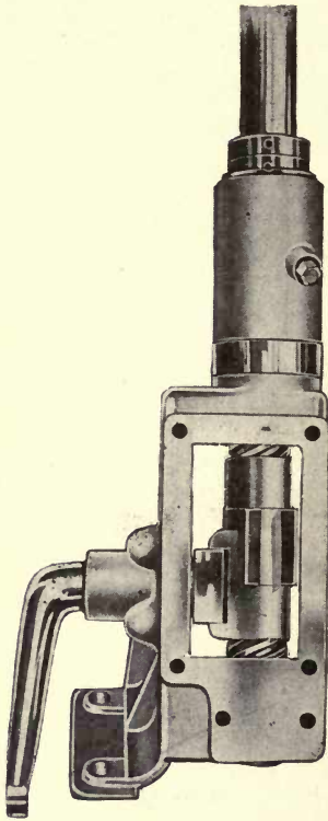
Fig. 24. Detail of Nut and Bell-Crank in Screw and Nut Type of Steering Gear. Knox Automobile Company, Springfield, Mass.
