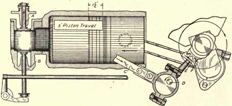
Fig. 28. Beginning of Second or Compression Stroke in a Four-Cycle Engine. Cadillac Motor Car Company, Detroit, Mich.
