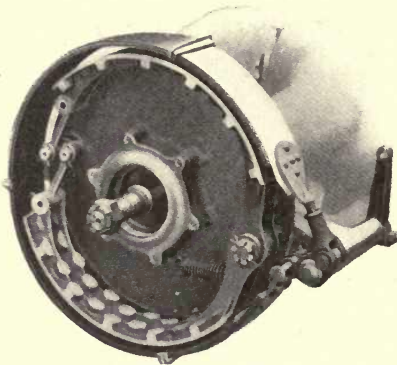
Fig. 121. Brake Drum. Showing detail of internal expanding and external contracting brakes. Premier Motor Mfg. Co., Indianapolis, Ind.
