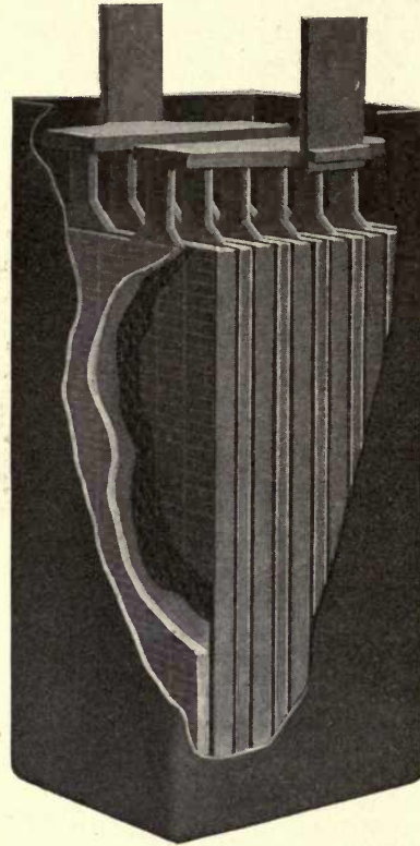
Fig. 143. Single Storage-Battery Cell. Universal Electric Storage Battery Company, Chicago, Ill.
