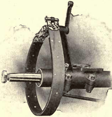
Fig. 95. Constriction-Band Clutch, as Used in Reo Car. Reo Motor Car Company, Lansing, Mich.
