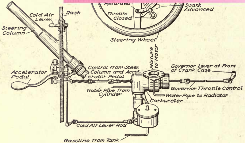
Fig. 91. Throttle-Control System of Peerless Car. Peerless Motor Car Company, Cleveland, Ohio.
