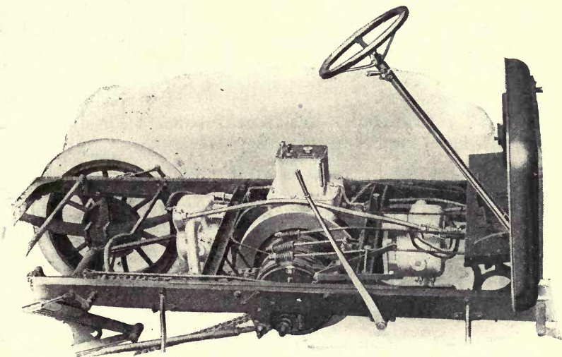
Fig. 96. Side View of Part of Chassis of Reo Car, Showing Constrictor-Band Clutches and Operating Rods. Reo Motor Car Company, Lansing, Mich.
