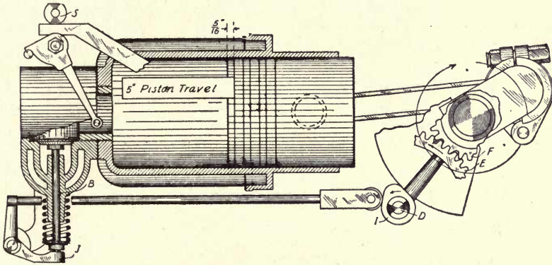
Fig. 29. End of Working or Third Stroke in a Four-Cycle Engine. Cadillac Motor Car Company, Detroit, Mich.
