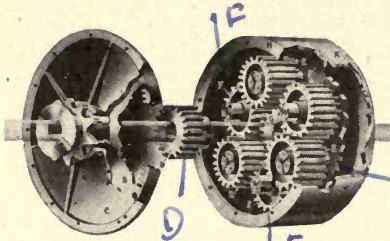
Fig. 101. Planetary Transmission Gear of Cadillac Single-Cylinder Car. Cadillac Motor Car Company, Detroit, Mich.
