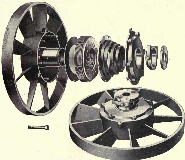
Fig. 99. Multiple-Disc Clutch of the Franklin Car. H. H. Franklin Manufacturing Company, Syracuse, N. Y.
