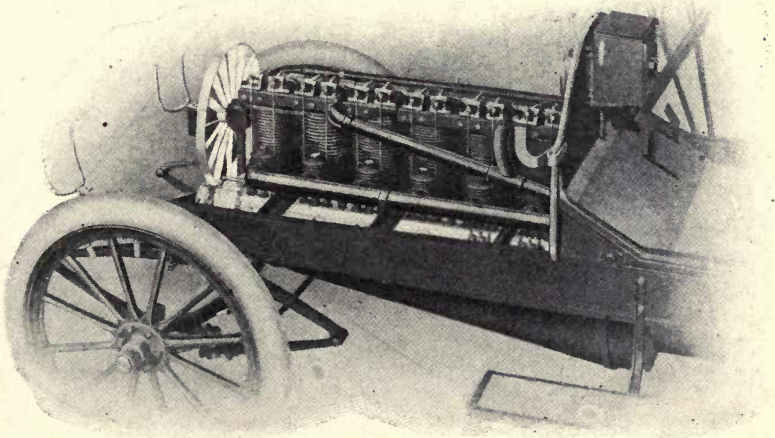
Fig. 50. Exhaust Side of Franklin Six-Cylinder Engine, Showing Regular Exhaust Pipe from Top and Auxiliary Exhaust from Bottom of Cylinders. H. H. Franklin Manufacturing Company, Syracuse, N. Y.
