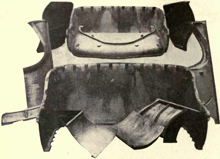
Fig. 5. Component Parts of an Aluminum Body. Nordyke & Marmon Company, Indianapolis, Ind.
