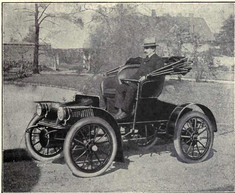
Fig. 153. Suburban Runabout. Baker Motor Vehicle Company, Cleveland, Ohio.—Mr. W. C. Baker, Designer of First Baker Electric, in Car.
