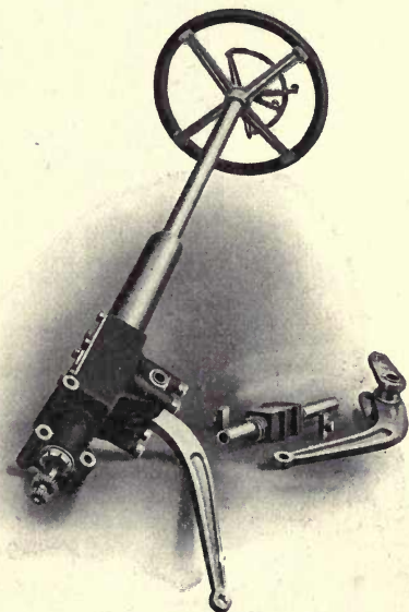
Fig. 23. Steering Column of Screw and Nut Type. Knox Automobile Company, Springfield, Mass.
