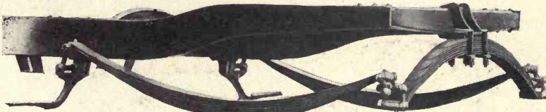
Fig. 10. Rear Spring Suspension. Peerless Motor Car Company, Cleveland, Ohio.
