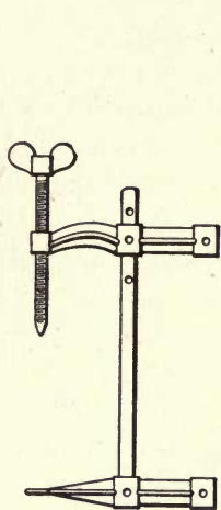
Fig. 44. Lifter Assembled.
