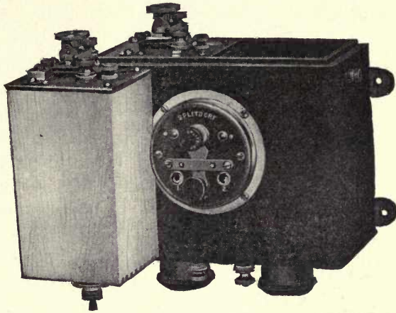
Fig. 74. Dash Coil for Two-Cylinder Engine. Cover Removed. Also note removable unit. The Splitdorf Laboratory, New York City.
