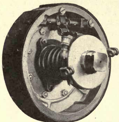
Fig. 97. Leather-Faced Disc Clutch. Peerless Motor Car Company, Cleveland, Ohio.
