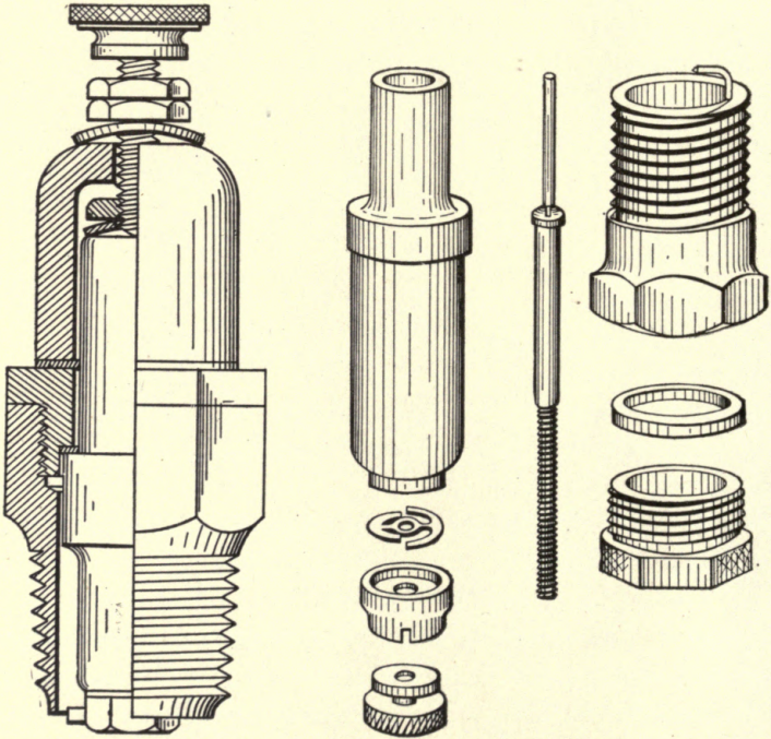
Fig. 84. Section of Sta-Rite Spark-Plug. R. E. Hardy Company, New York, N. Y.
