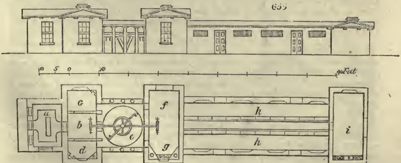
(a, b, c, d), is at the north end, has hollow walls, double doors, double sashed windows and an ice-house under. The milk room (a), is surrounded by milk coolers, and has a butter slab and jet in the centre. The jet is supplied from a cistern over the steaming,
