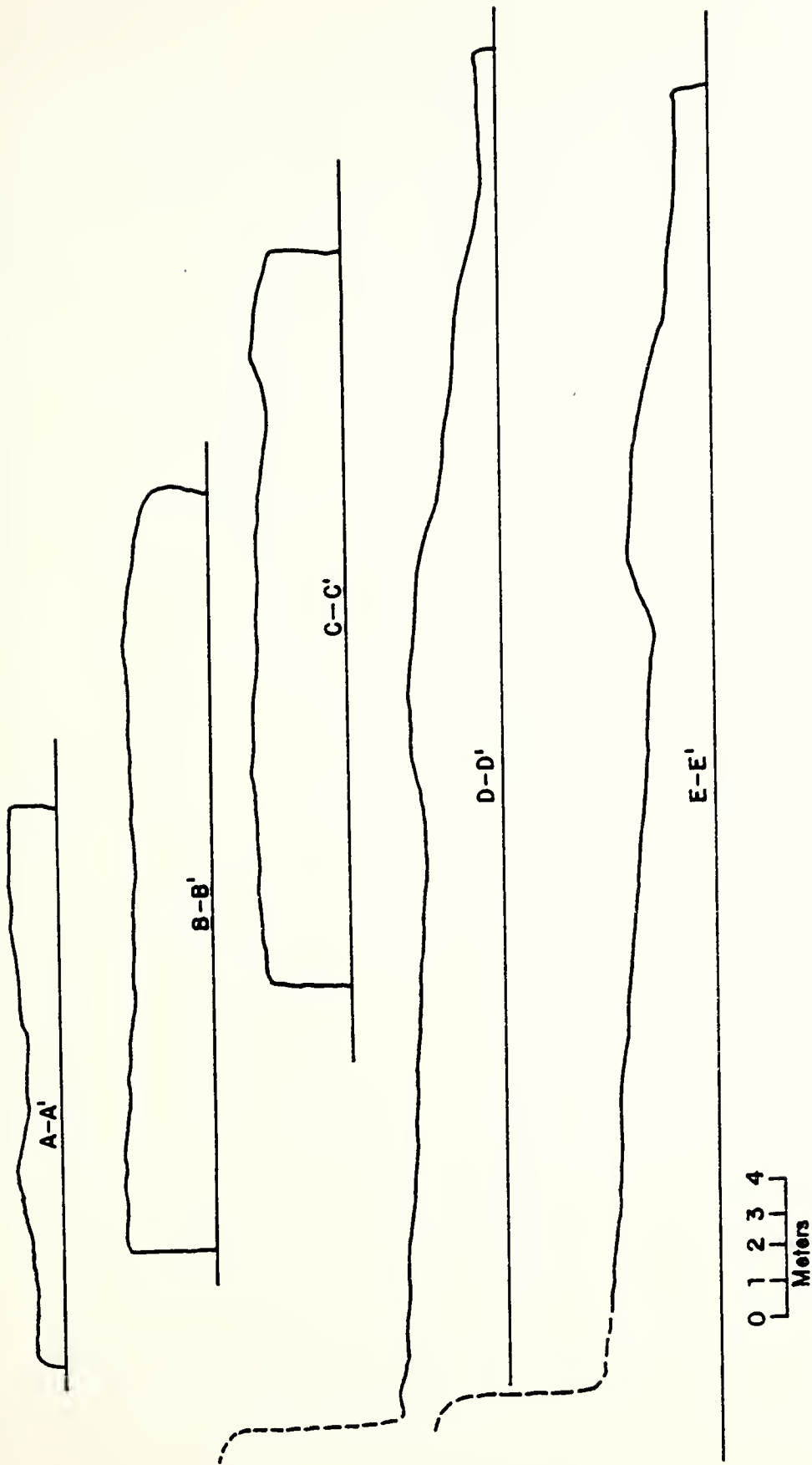
Figure 4. Cross-sectional profiles through primary reef area.
