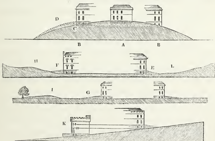
[Fig. 24. Sections to shew the manner of adapting houses to different natural shapes of ground.]
