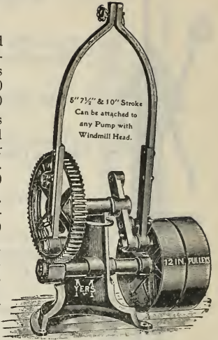
Fig. 1114, Pump Jack
