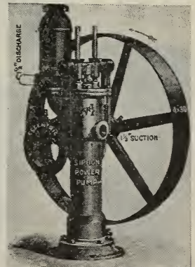
Fig. 1226 Power Siphon Pump
