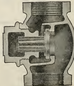
Horizontal Check Valve
