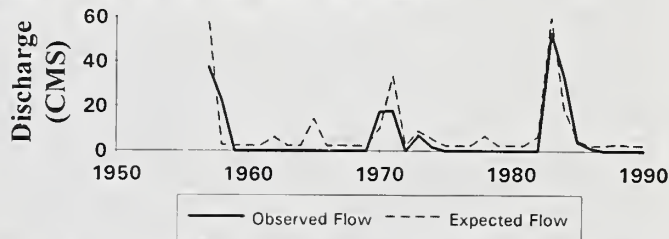
Figure 8. — Comparison of observed and expected flow equal to or exceeding bankfull at St. Louis Creek for the post diversion period 1957 - 1990.
