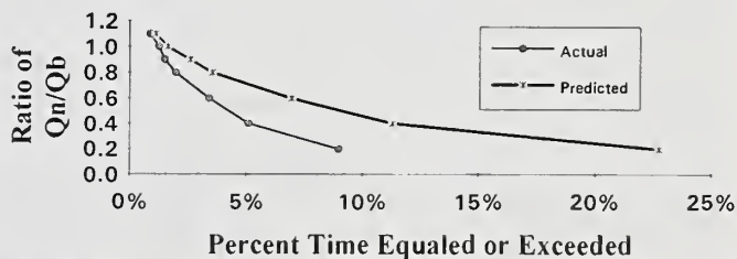
Figure 9. — Flow duration curve for St. Louis Creek (1967-1990) comparing the mean duration predicted from East St. Louis Creek vs. the actual mean.
