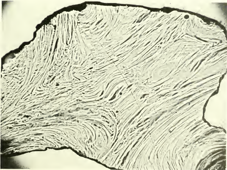
1. Moldavite, illustrating the inhomogeneity of a thin polished section by means of transmitted light.
