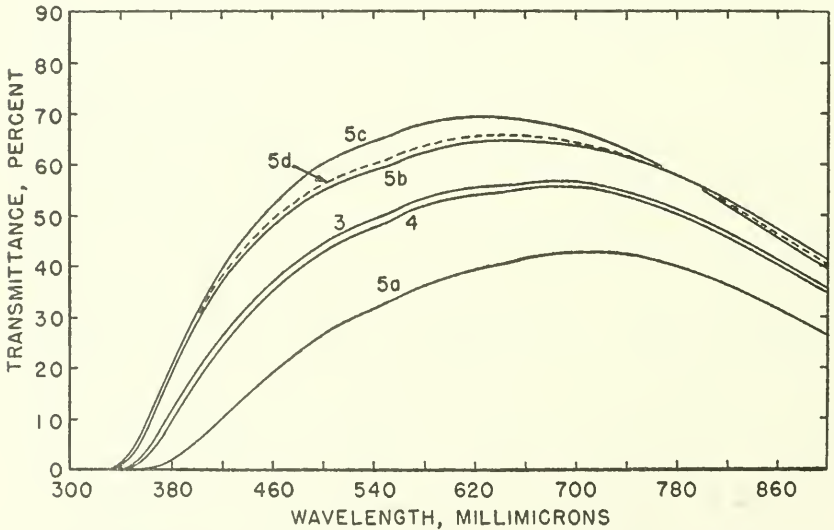
FIGURE 2.—Spectral transmittances of six bediasites from Texas: No. 3, near Muldoun, Fayette County; No. 4, eastern portion of Lee County; Nos. 5a, 5b, 5c, and 5d, near Bedias, Grimes County. Courtesy of Virgil E. Barnes, University of Texas.
