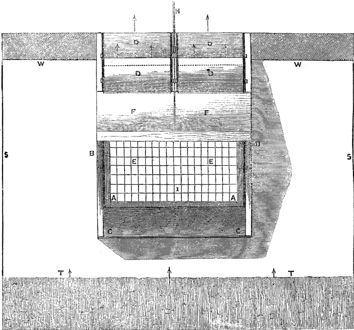
Fig. 15. Bird's-eye view.
