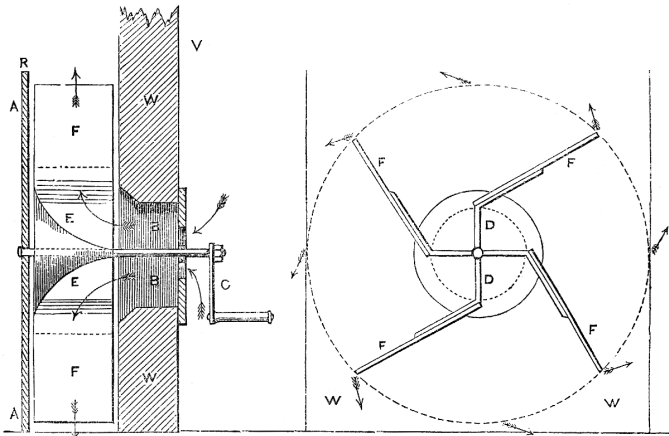
Fig. 17. Front view, the frame being removed.
