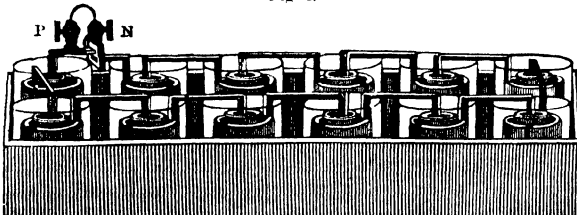
A battery formed of twelve cups on the plan of Mr. Grove. P. Positive pole. N. Negative pole. W. Wire.
