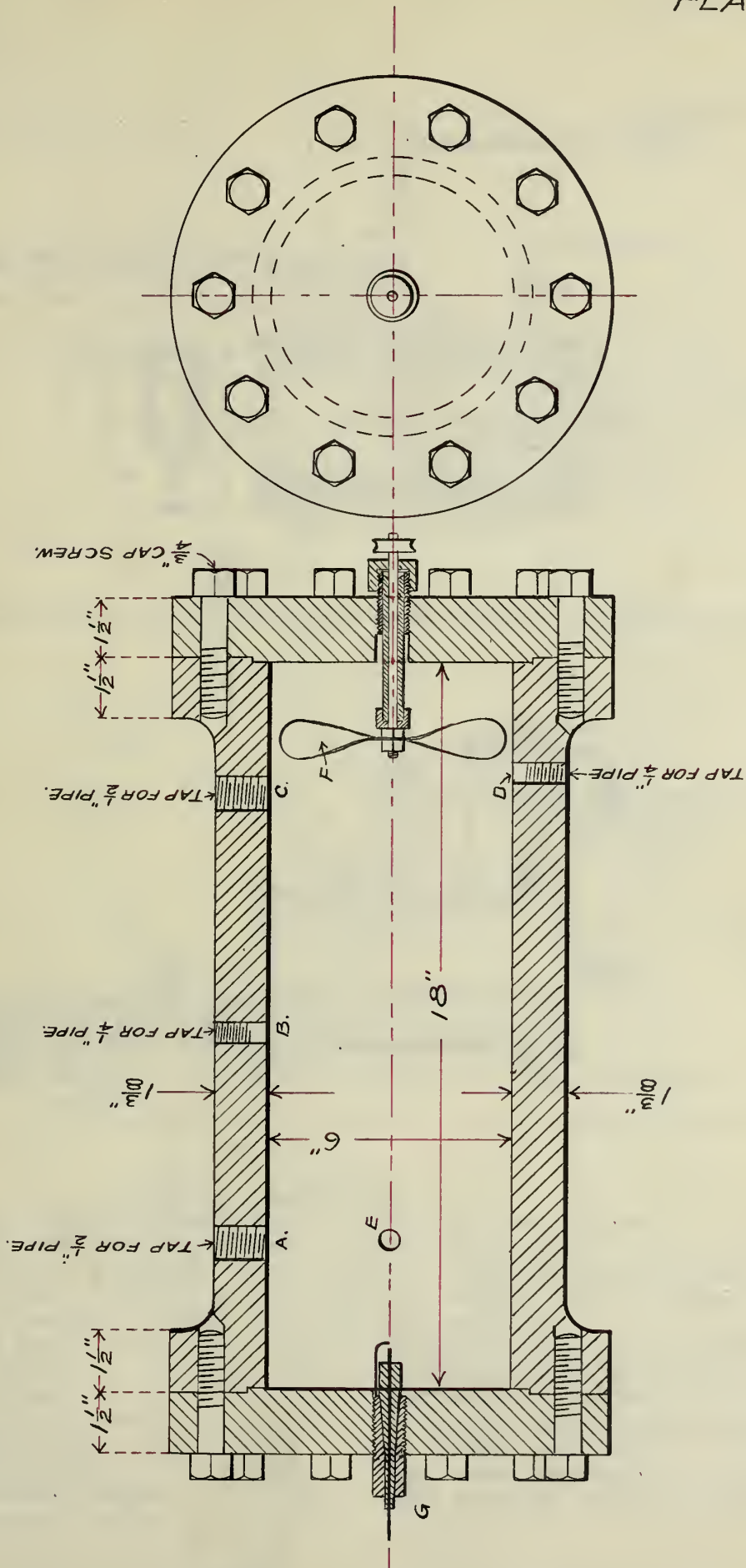
CAST IRON EXPLOSION CYLINDER. SCALE 1" = 4"
