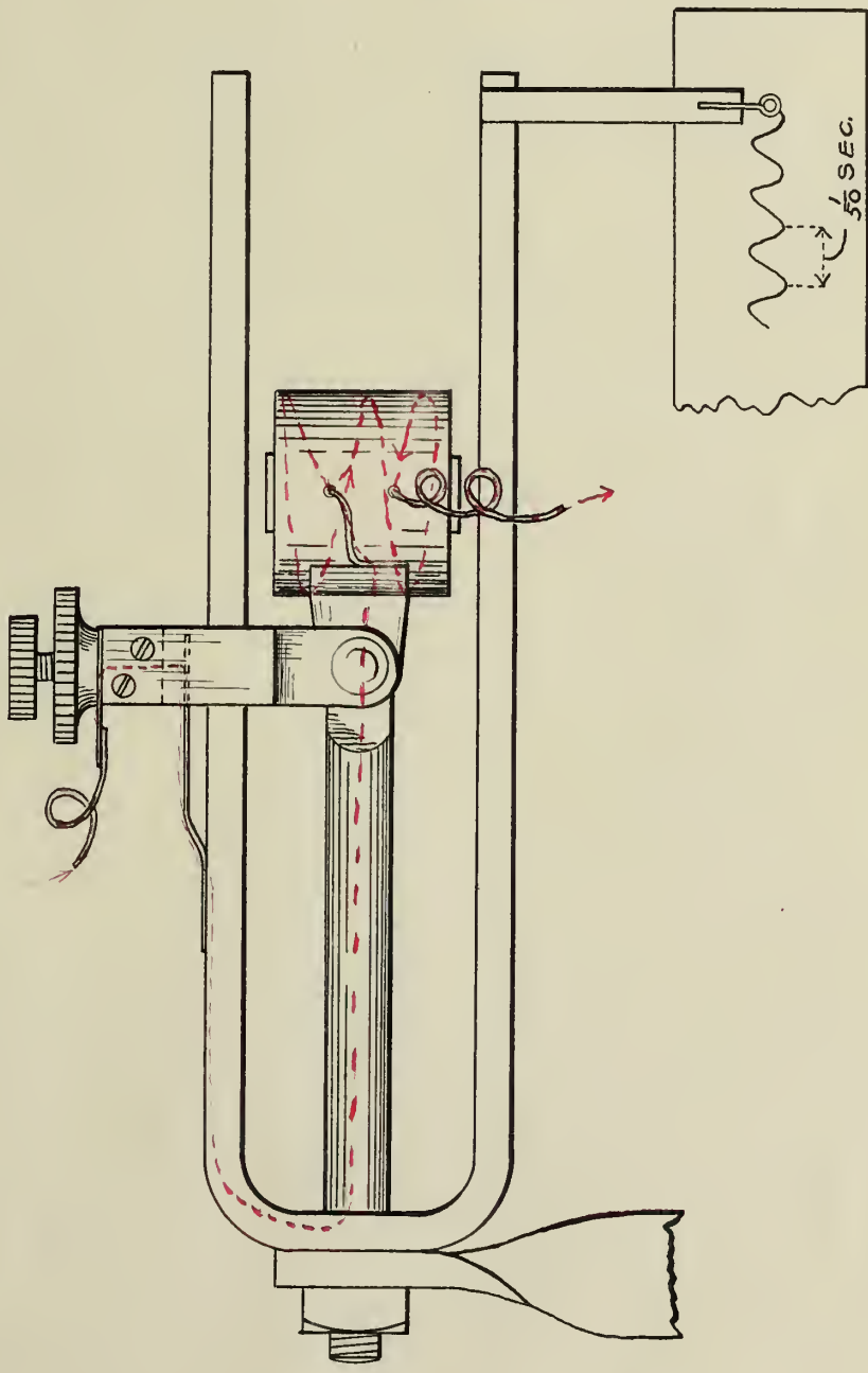
ELECTRICALLY OPERATED TIMING FORK. CURRENT FOLLOWS PATH SHOWN IN DOTTED RED.
