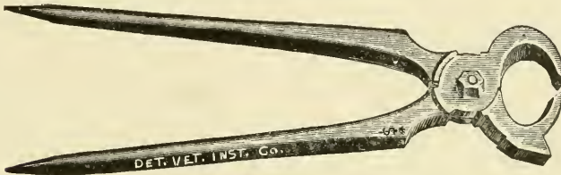
FIG. 35.—Iron pinchers for removing sole and wall of hoof.
