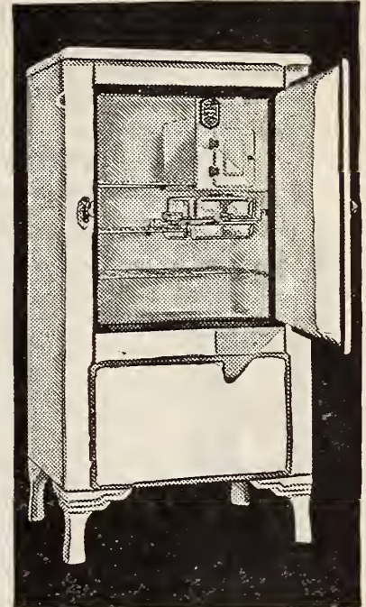
The Guardian—Model 71: Capacity, 7.53 cu. ft.; Shelf area, 11.35 sq. ft.; Ice, 4 trays, 21 cubes each, total 84. Finish: Exterior and Interior, Porcelain. Height, with 8½ in. legs, 61¼ in.; width, 32½ in.; depth, 25¾ in. Watervoir shown in this model is extra equipment.
