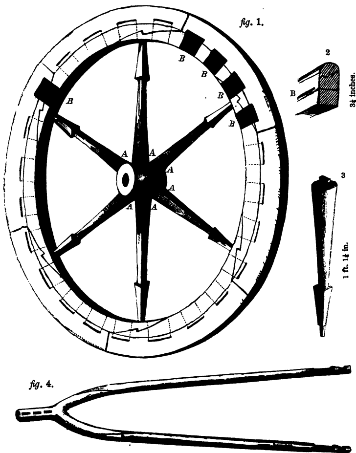
Fig. 1. Wheel; 3 ft. 1 in. diameter. In the Collection of Dr. Abbott. Fig. 4. Shafts; 11 feet in total length.
