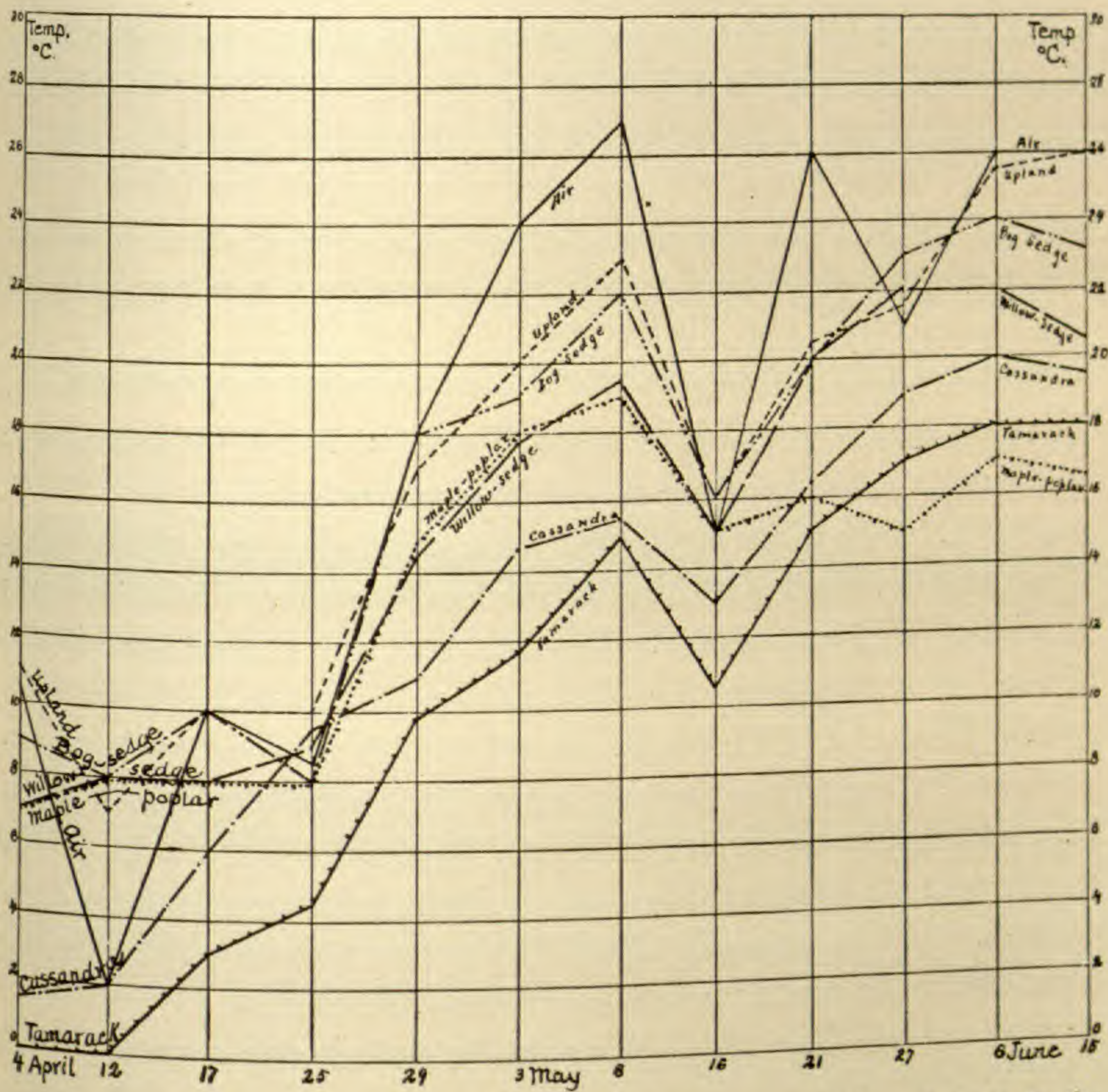
FIG. 5.—Diagram showing temperatures of the air and the substrata in the several plant societies.
