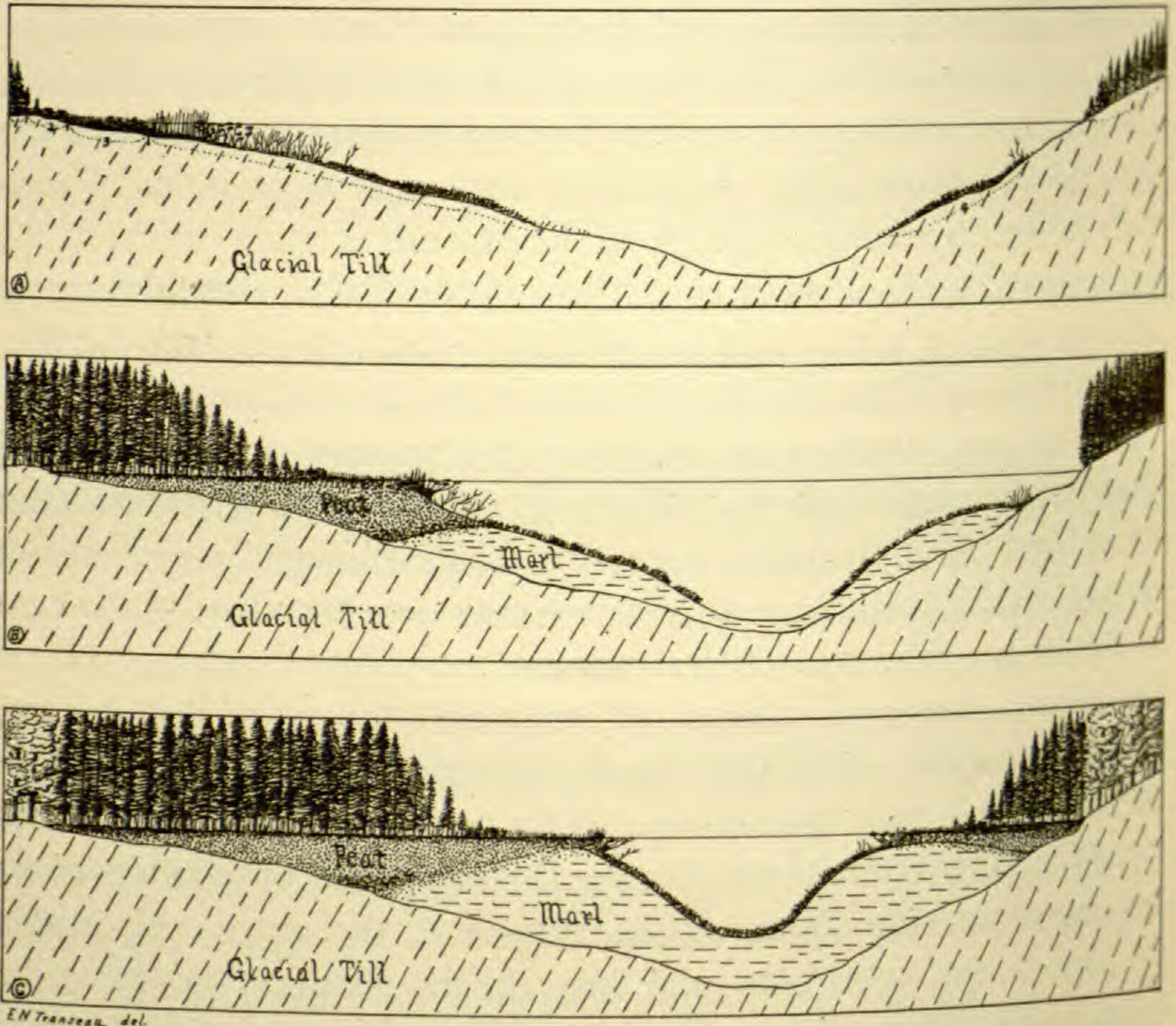
FIG. 4.—Diagrams illustrating three stages in the development of peat and marl deposits in lake basins. In drawing the figures it has been assumed that the rates of marl and peat deposition are approximately equal. The peat accumulates most rapidly on the western side of the basin. On the east side a common effect of wave action is illustrated. The process of peat formation is hindered, while that of marl deposition goes on until the aggradation of the bottom reduces the force of the waves sufficiently to allow the bog plants a foothold. A represents conditions in early postglacial times when these basins acquired their first flora. The several plant societies represented are (1) conifer (2) bog shrub, (3) bog sedge, (4) aquatic, the outermost division of which is the chara association. In B the conditions for the growth of plants belonging to the northeastern conifer forest formation have reached their optimum. C represents present conditions in southern Michigan. The plants belonging to the southeastern broad-leaved forest formation, being climatically favored, occupy the areas of mineral soils, while the conifers are almost restricted to bog areas.
