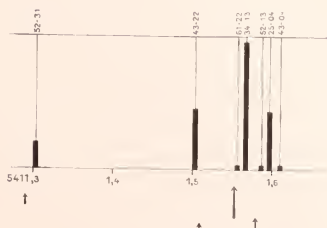
Fig.12 5411 Å (helium), (7-4).
