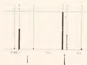
Fig.13 6562 Å (hydrogen, H_{\alpha} ), (3-2).
