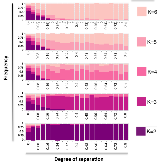
c) CLEST
