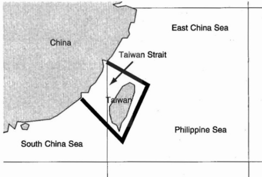
FIGURE 2.1 Taiwan Strait.
