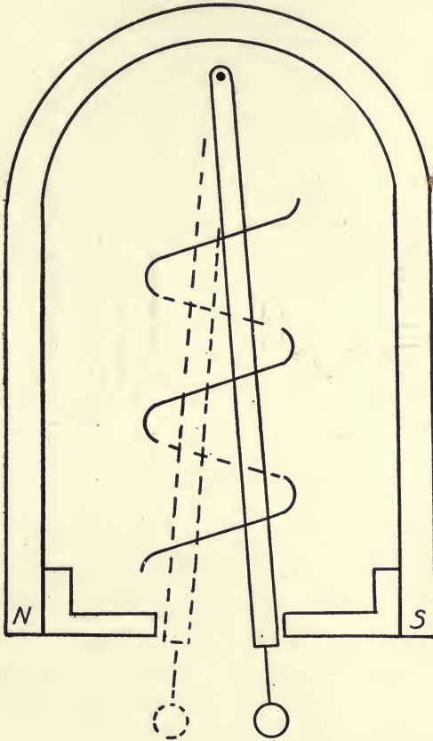
FIG. 73.—POLARIZED MECHANISM Single coil and soft-iron vibrator
