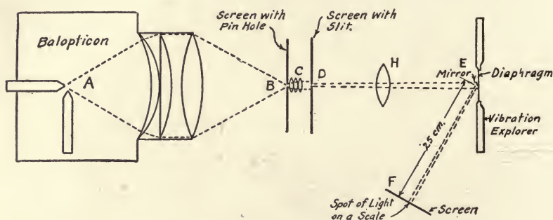
FIG. 20.—OPTICAL SYSTEM FOR VIBRATION EXPLORER (Kennelly and Taylor)
