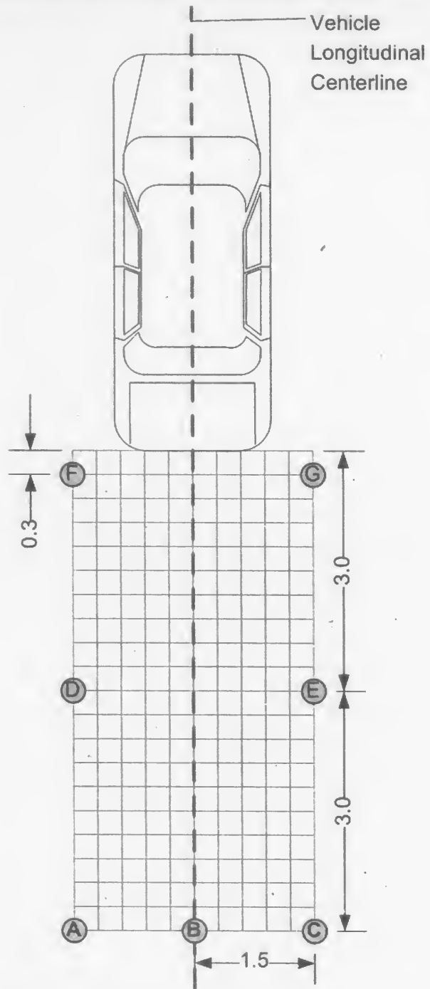
FIGURE 5: TEST CYLINDER LOCATIONS (Units in meters)
