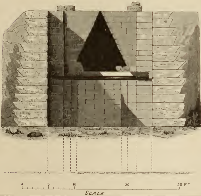
FAÇADE, PLAN, AND SECTION OF THE TREASURY NEAR THE LIONS' GATE.
