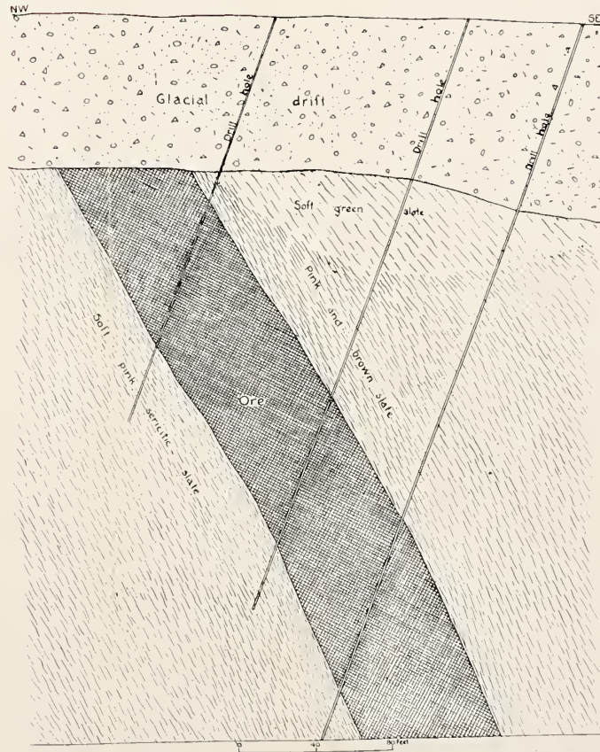
TYPES OF ORE DEPOSITS IN THE CUYUNA IRON-ORE DISTRICT MINNESOTA
