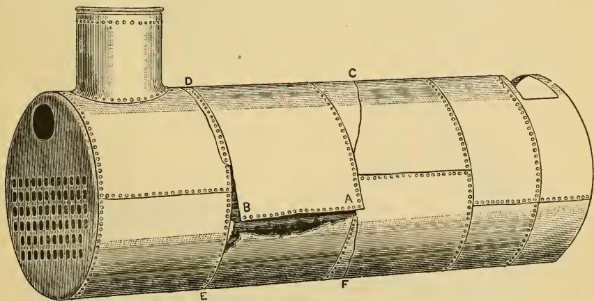
FIG. 1.—BA, line of initial fracture; AC, AF, BE, and BD, lines of secondary fracture, being the boundary lines of the detached ring of plates.
