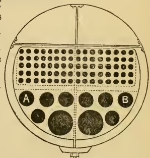
FIG. 3.—Section through the back smoke chamber giving a rear view of the rear tube plate, with the ruptured tube omitted. A and B the ruptured 10-inch flues.
