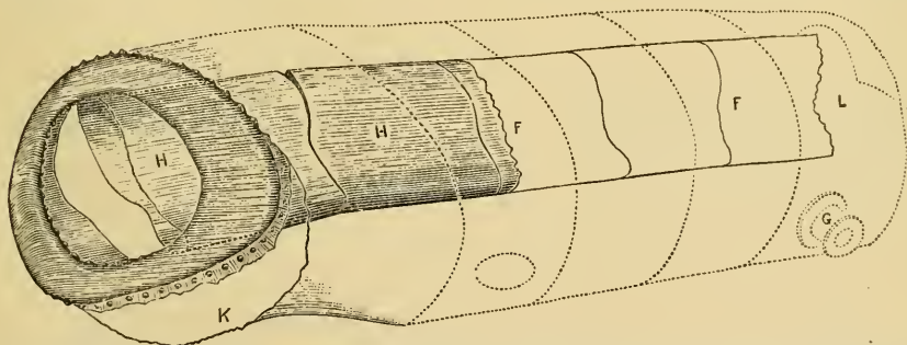
FIG. 1.—The dotted lines represent the unbroken part of the shell. The shaded portion at the left shows the foremost parts of the shell broken by the fall. The shaded portion of the flue remained in the shell, and that portion in flue outlines was blown out with the missing portion of the head at the right.
