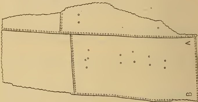
FIG. 2.—Ring of plates broken off by the force of the escaping water and steam.
