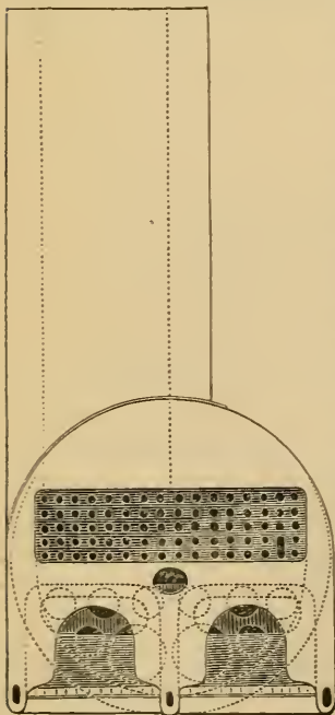
FIG. 2.—Front elevation of the boiler, showing the opening in the tube plate made by the boiler-maker shortly after the accident, for the purpose of removing the ruptured tube, which was the lowest one of the second vertical row from the right hand.
