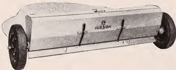
Judson All Steel Broadcaster is built in 8 foot width and 12 bushel capacity. Equipped with wheels for rubber tires, roller bearings, rotary wing force feed and divided axle, enabling operator to run one-half machine independent of other.
