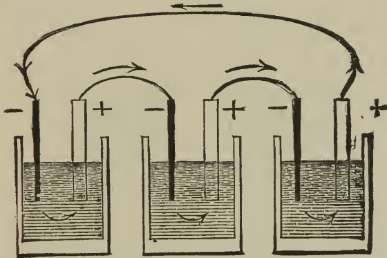
FIG. 138.—A COMPOUND CHAIN. (After Erb.) Three sets of elements are here connected "behind one another," or "in series." The direction of the current is shown by the arrows. The circuit of closure is effected by a wire, as in Fig. 137, B.
