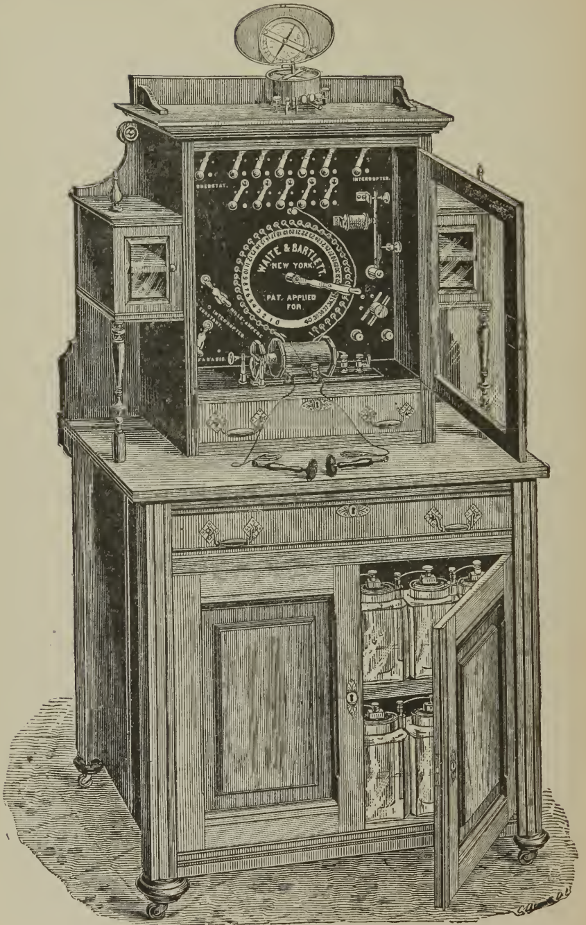
FIG. 162 —THE PERFECTED OFFICE CABINET BATTERY. (Author's model.)
