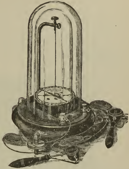
FIG. 156.—THERMO-ELECTRIC DIFFERENTIAL CALORIMETER.—Connect the two thermostats as shown in figure, viz : connect by means of one of the metal-tipped cords one binding-post of each of the thermo-piles to the two binding-posts on base of the galvanometer. Then connect the two remaining posts, one on each of the thermo-piles with each other. After so doing, place the thumb on the face of one of the thermo-piles and observe the direction of the deflection of the galvanometer-needle, then place thumb on face of the other thermo-pile, leaving the first uncovered, and, if the deflection is in the opposite direction to that first obtained, the instruments are properly connected. If, however, the second deflection is in same direction as obtained by pressing thumb on first thermo-pile, disconnect the two cords from either thermo-pile and interchange them, viz : take cord from right-hand post and place in left, and cord from left post and place in right hand post; the deflections will then be as first alluded to, one pile turning needle in one direction and the other in the opposite direction.
