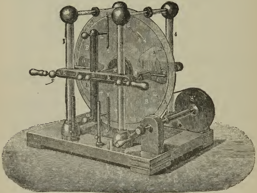
FIG. 171.—THE ORIGINAL MODEL OF HOLTZ'S INDUCTION MACHINE WITH VERTICAL PLATES. The same inventor also perfected a machine without windows or armatures, in which two horizontal plates revolved in opposite directions. This machine is shown in a subsequent cut.
