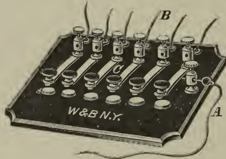
FIG. 60.—THE AUTHOR'S DIAGNOSTIC KEY-BOARD.— A , the rheophore which connects it with one of the binding-posts of a galvanic battery; B , rheophores connecting its binding-posts with spring electrodes previously placed upon the body of the patient so as to influence the nerves or muscles to be tested; C , buttons and springs which make a circuit to the body of the patient when the knob on the spring is pressed downward so as to impinge upon the button. The number of rheophores which may be employed depends upon the necessities of the case; the cut shows an instrument capable of six.
