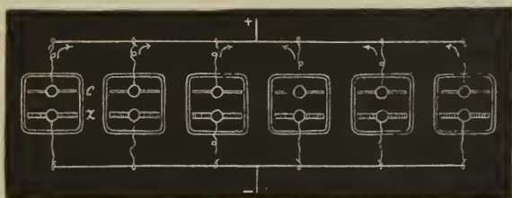
FIG. 141.—SIX CELLS CONNECTED FOR QUANTITY, i.e. , "in surface," or in "simple circuit." (After De Watteville.) z, zinc elements; c, carbon or platinum elements. This arrangement does not affect the "electro-motive force" of the battery.
