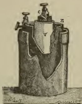
FIG. 149.—BUNSEN'S CELL.—Parts are represented as bitten away to show its arrangement: the cylinder of zinc ( z ); a porous cup ( v ); and the carbon ( c ) within it. This cell is not employed in medical batteries, for reasons similar to those given in connection with Fig. 148.
