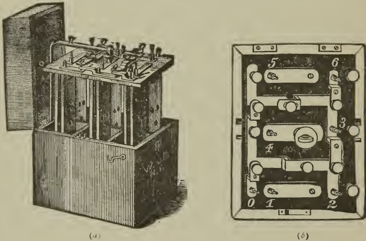
FIG. 188.—PIFFARD'S CAUTERY BATTERY.—(a) The battery as suspended when not in action. (b) Arrangement of the top of this battery, showing the screws which regulate the connections between the different cells. The battery is rocked during its action to prevent extreme polarization. By making the movement slow or rapid, the heat of the loop or knife may be regulated at will.
