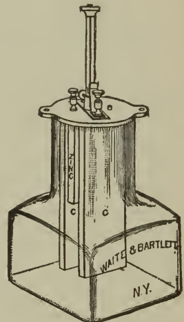
FIG. 144.—GRENET'S CELL.—The flasks come of all patterns, according to the taste of the various makers. In the form here depicted the zinc is lowered into the fluid by a straight handle. This is the cell most used in portable electrical apparatus. It is cheap, efficient, and easily repaired. Removing the elements and replacing them overcomes “polarization” in case the current grows weak from that cause. Some makers place the zinc in a drip-cup when the cell is not in use.
