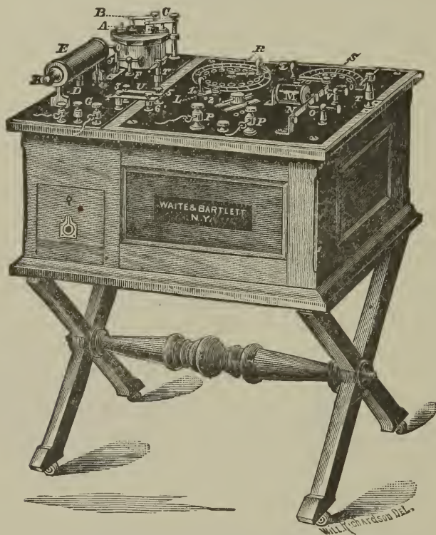
FIG. 161.—THE PHYSICIAN'S HANDY CABINET BATTERY. ( Author's model .) The accompanying cut represents a light and compact form of cabinet battery, designed by the author. It is on castors, and can be wheeled about the consultation-room. This admits of the use of the instrument when the patient is in the gynæcological chair or upon the office lounge; or when any form of fixed apparatus, such as the laryngoscope, the inhaler or spray, etc., is being simultaneously employed. In some of my later models an immovable tray is placed beneath the battery for electrodes, and a movable shelf is also provided upon which a milliampère-meter, the solution of table salt, and the electrodes in actual use can be set. A glass cover protects the battery from dirt when not in use. E , faradaic coils; K , plunger; G , faradaic binding-posts; F , interrupter; D , drip-cup; R , current-selector of single cells; S , the same of four cells to each button; M , coil to work the interrupter for the galvanic current; L , switch to work or disconnect the interrupter ( V ); P , galvanic binding-posts; 3-3 and 4-6, connecting rods to allow of the action of M . The commutator lies above P .
