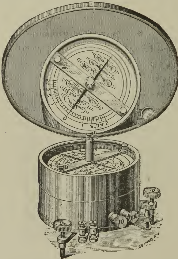
FIG. 153.—“DEAD-BEAT” MILLIAMPERE-METER.
