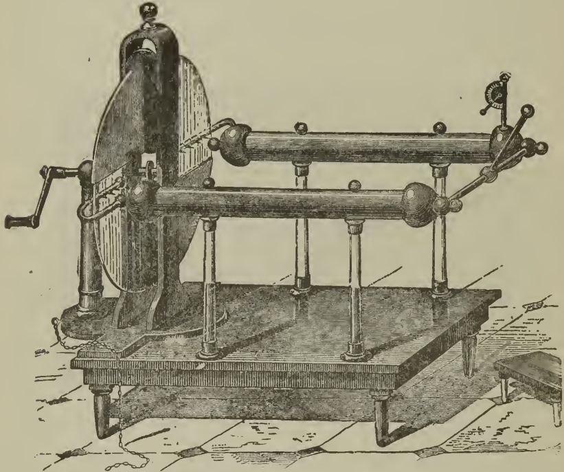
FIG. 165.—RAMSDEN'S ELECTRICAL MACHINE. (Invented in 1768.) It has sector-shaped pieces of oiled silk to prevent a loss of electricity from the glass plate while passing from cushion to cushion.
