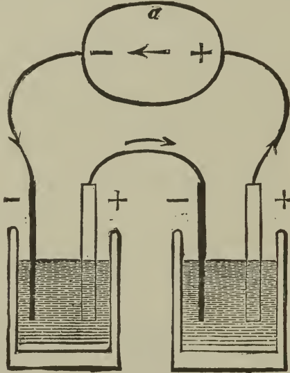
FIG. 139.—A SCHEMATIC REPRESENTATION OF THE INTRODUCTION OF A HUMAN BODY ( \alpha ) INTO THE CIRCUIT OF CLOSURE OF A GALVANIC CHAIN. (After Erb.) + = the anode; — = the cathode.
