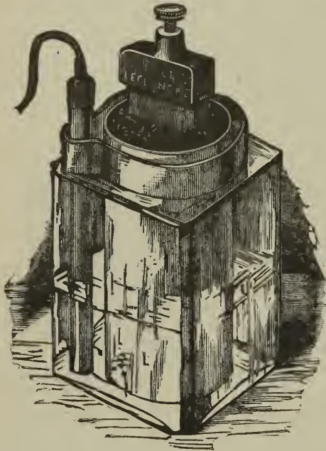
FIG. 143.—LECLANCHE'S CELL.—The zinc rod (the one with its rheophore attached) is shown as immersed in a solution of ammonic chloride. The carbon element is seen to project slightly above the porous cup, in which, when the cell is properly prepared for action, it is packed with peroxide of manganese and afterward covered with pitch.
