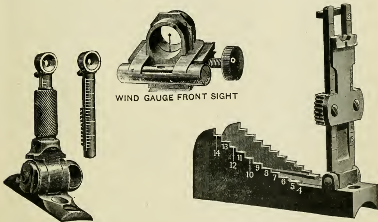
COMBINATION REAR SIGHT
