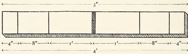
BED MARKER, OR MARKING BOARD
