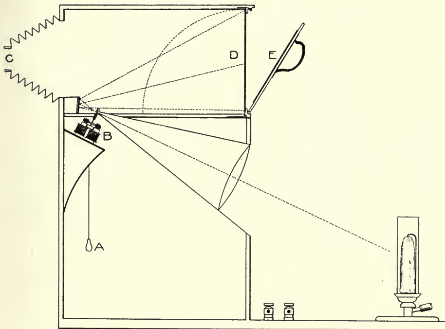
TACHISTOSCOPE
