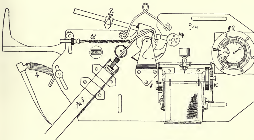
ERGOGRAFH (BACK VIEW)
