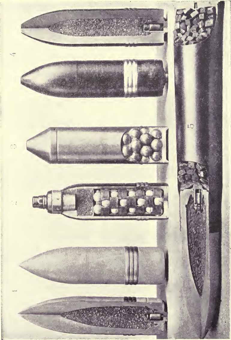
RAPID-FIRE AMMUNITION. (LXXIX)
