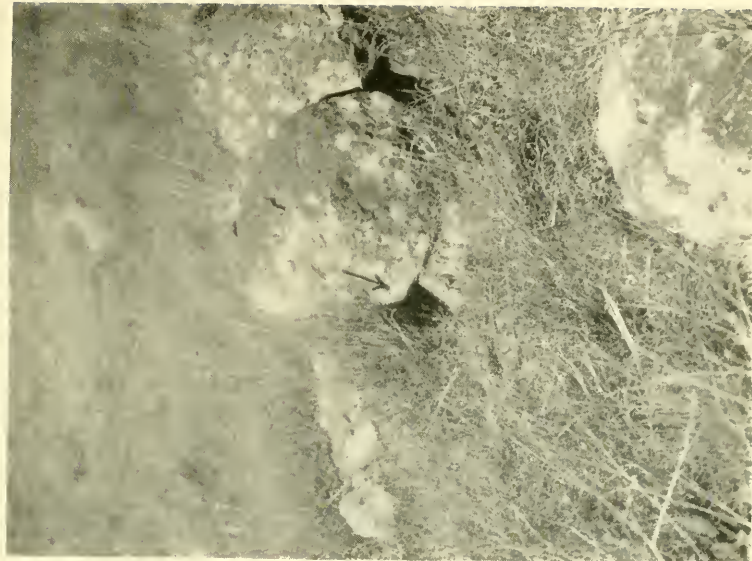
B Entrance to nest of Seebohm's wheatear ( Saxicola o. seebohmii ), four young, three-quarters grown, May 30. Plateau of Middle-Atlas (6200 ft.)
